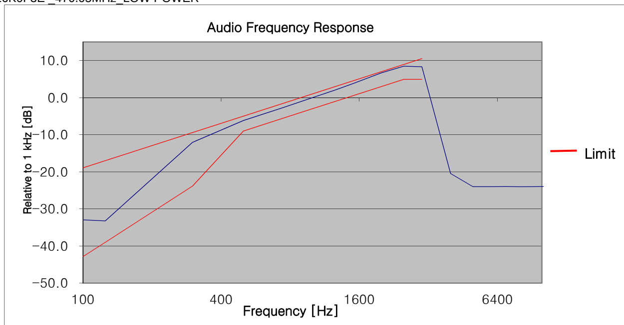
16K0F3E_470.05MHz_LOW POWER
