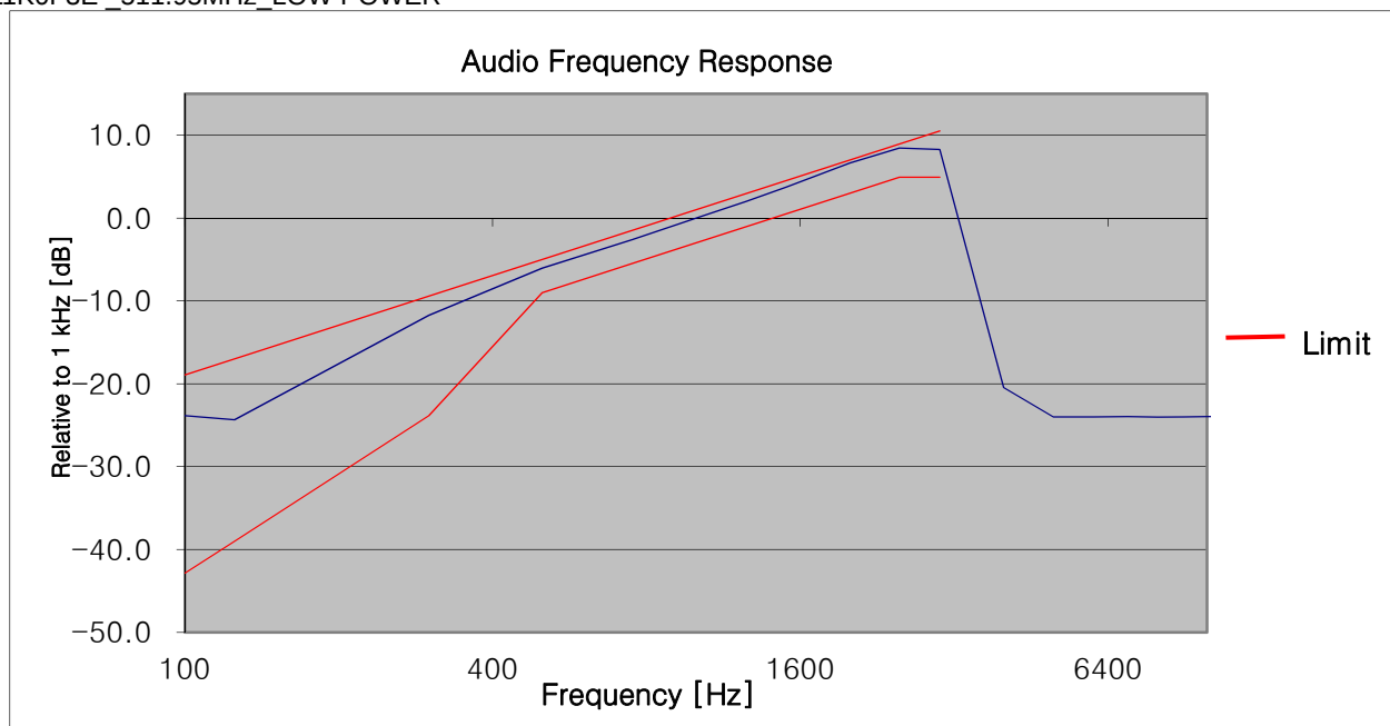
11K0F3E_511.95MHz_LOW POWER
