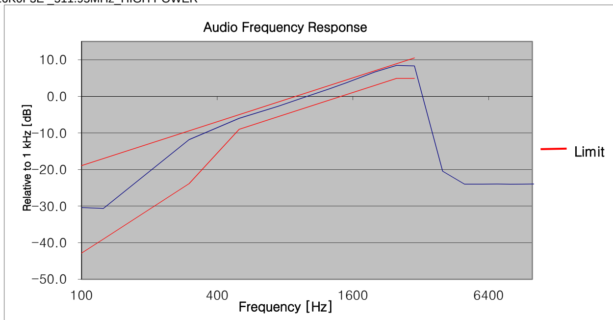
16K0F3E_511.95MHz_HIGH POWER
