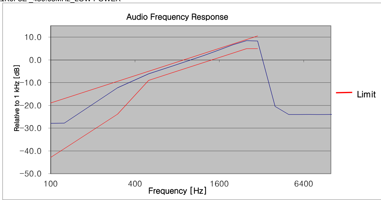
11K0F3E_450.05MHz_LOW POWER
