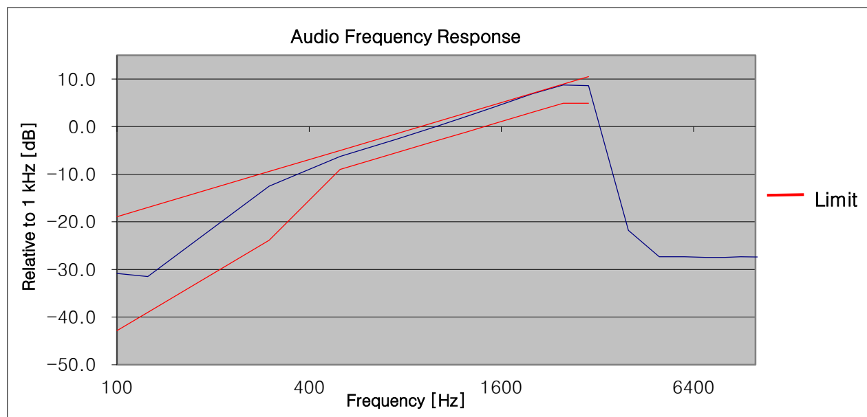
16K0F3E_162.05MHz_HIGH POWER
