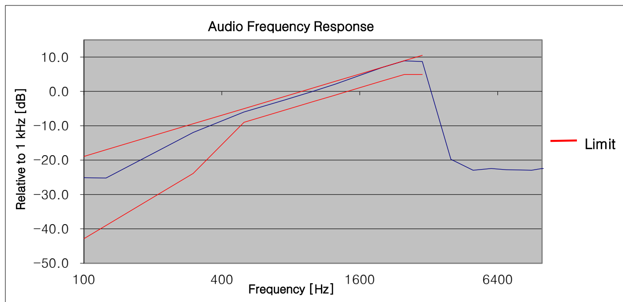
11K0F3E_162.05MHz_LOW POWER
