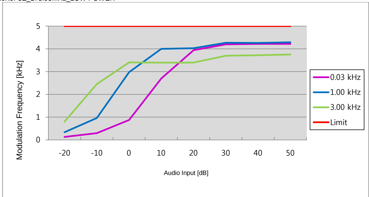
16K0F3E_173.95MHz_LOW POWER
