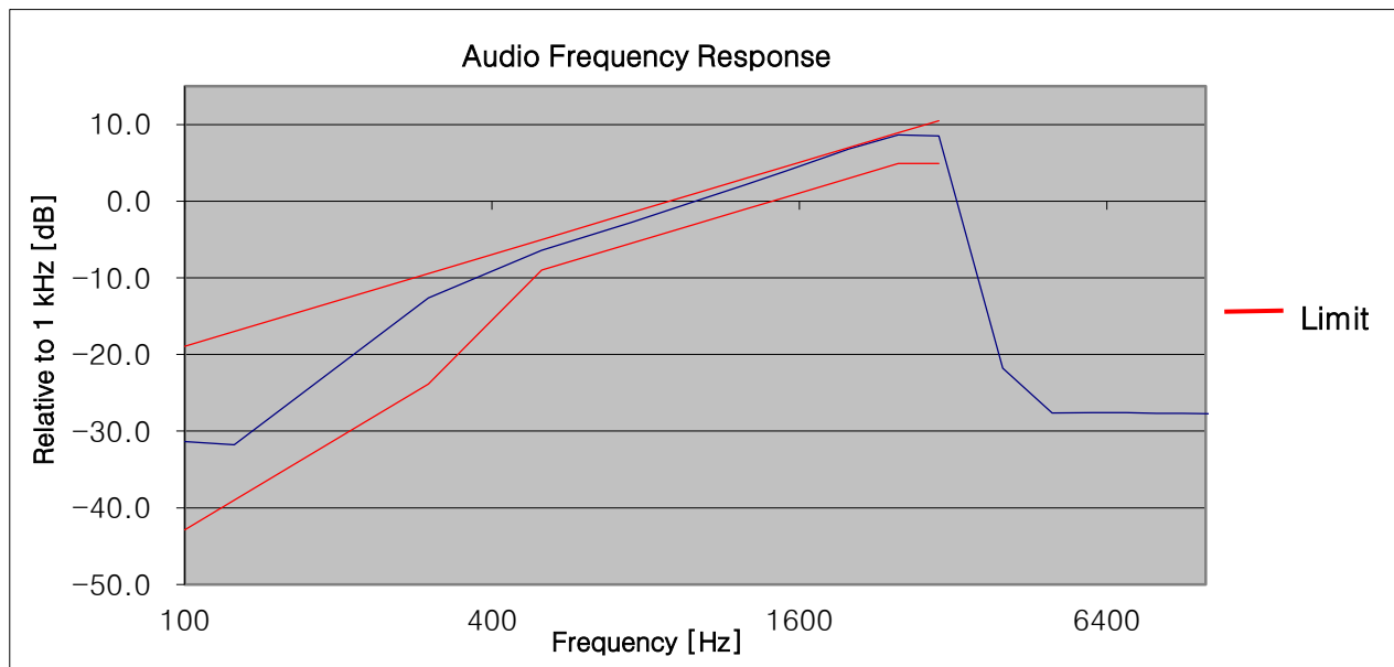
16K0F3E_173.95MHz_LOW POWER
