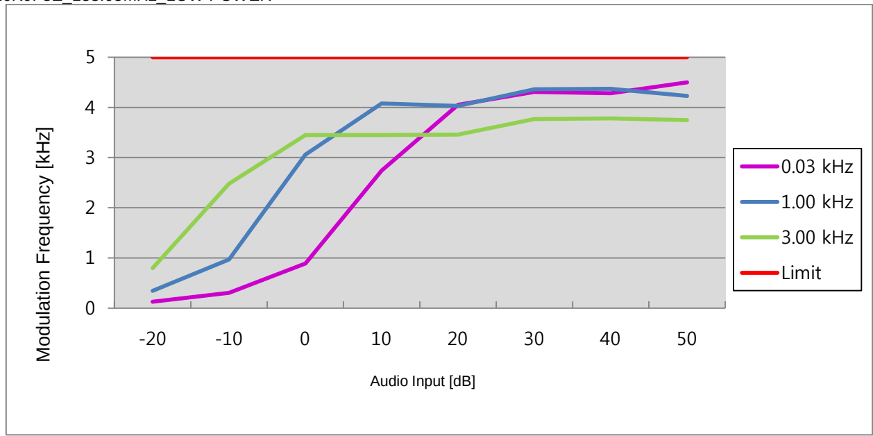
16K0F3E_138.05MHz_LOW POWER
