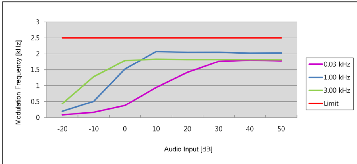
11K0F3E_173.95MHz_LOW POWER
