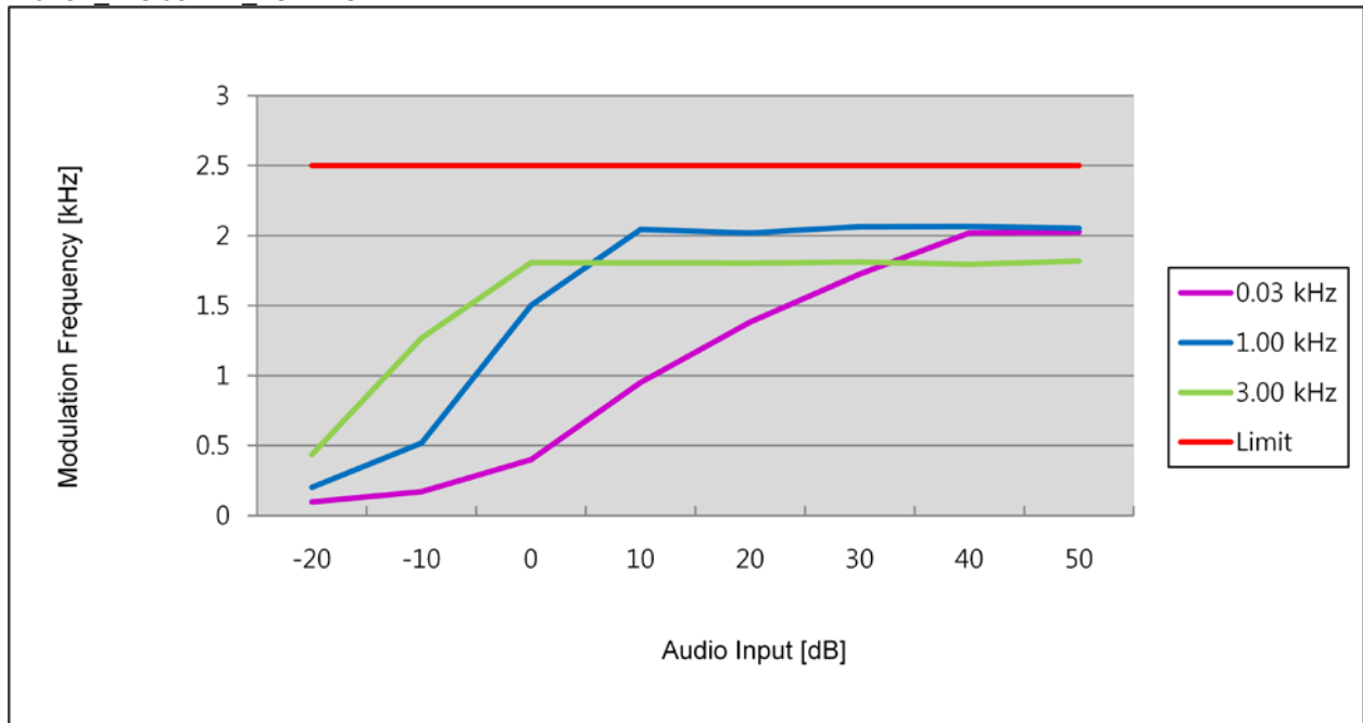
11K0F3E_173.95MHz_LOW POWER
