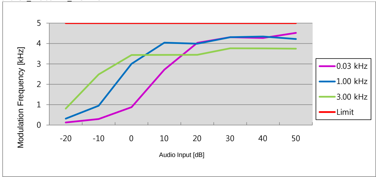
16K0F3E_173.95MHz_HIGH POWER
