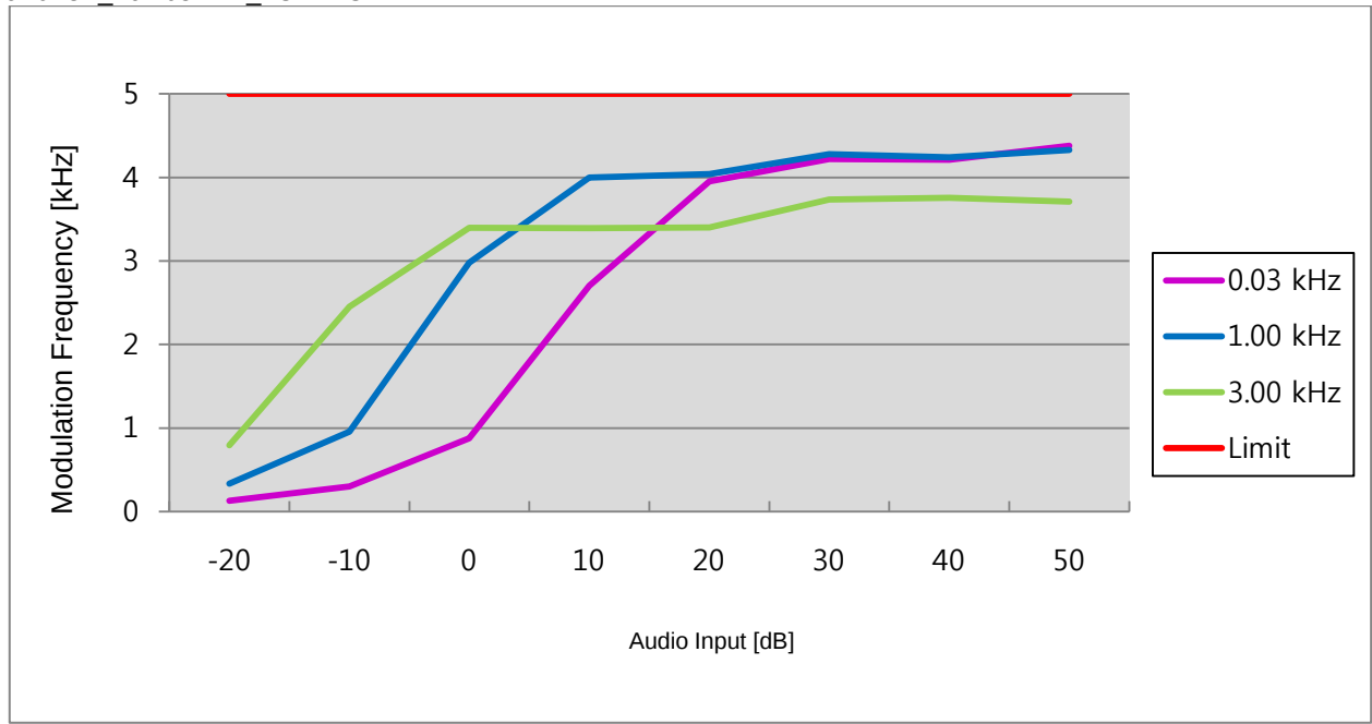
16K0F3E_162.05MHz_LOW POWER
