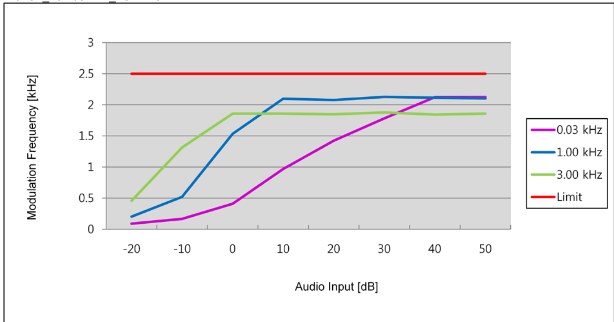
11K0F3E_162.05MHz_LOW POWER
