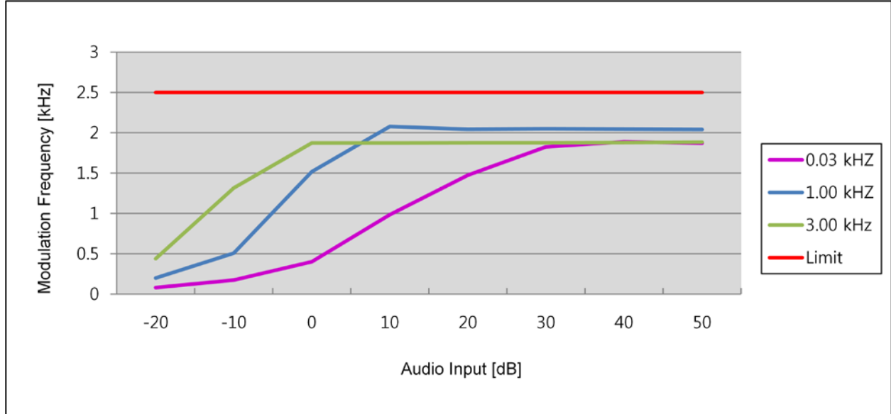
11K0F3E_138.05MHz_HIGH POWER
