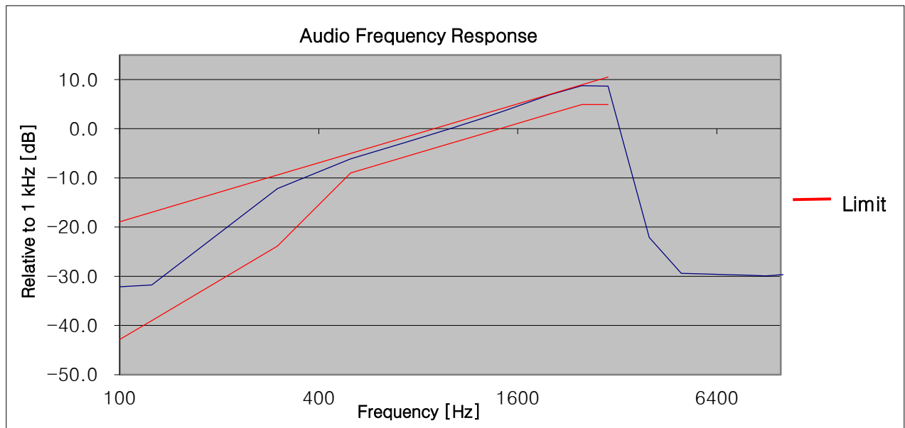
16K0F3E_138.05MHz_HIGH POWER
