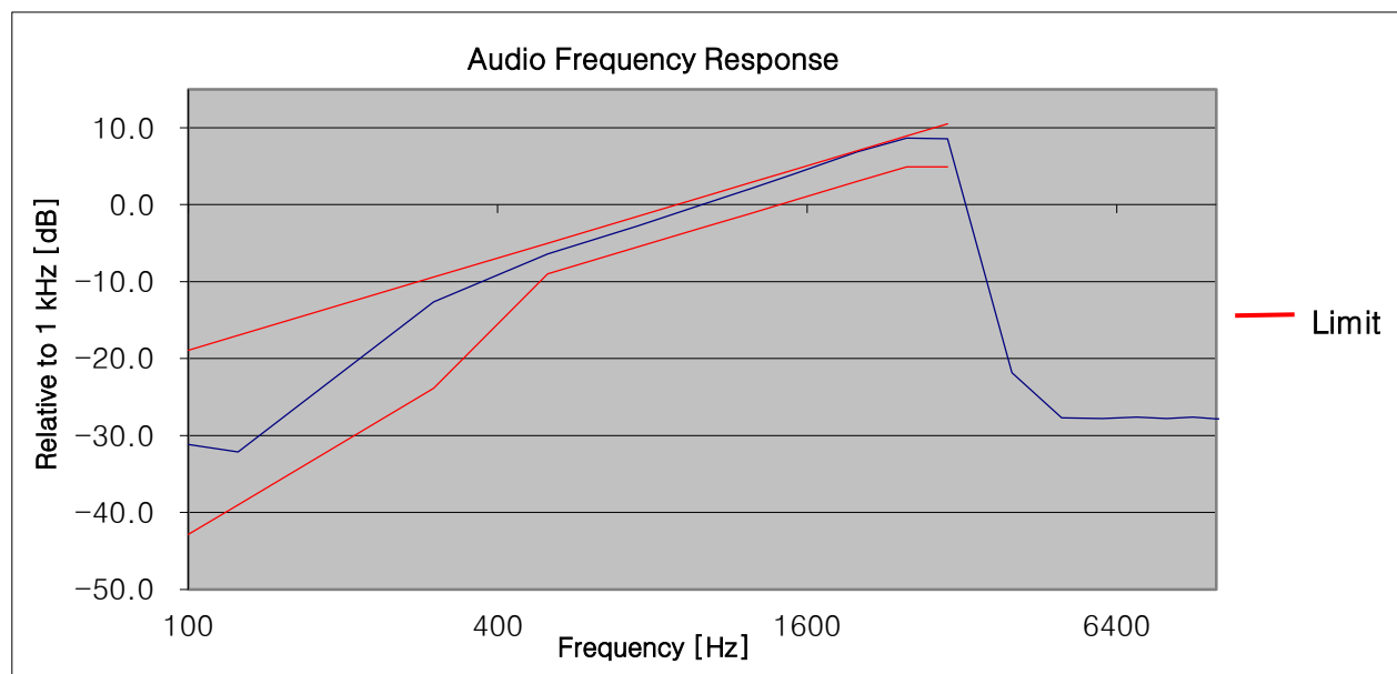
16K0F3E_173.95MHz_HIGH POWER
