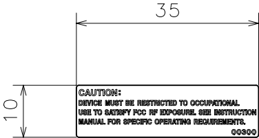
SCALE(1:1)
