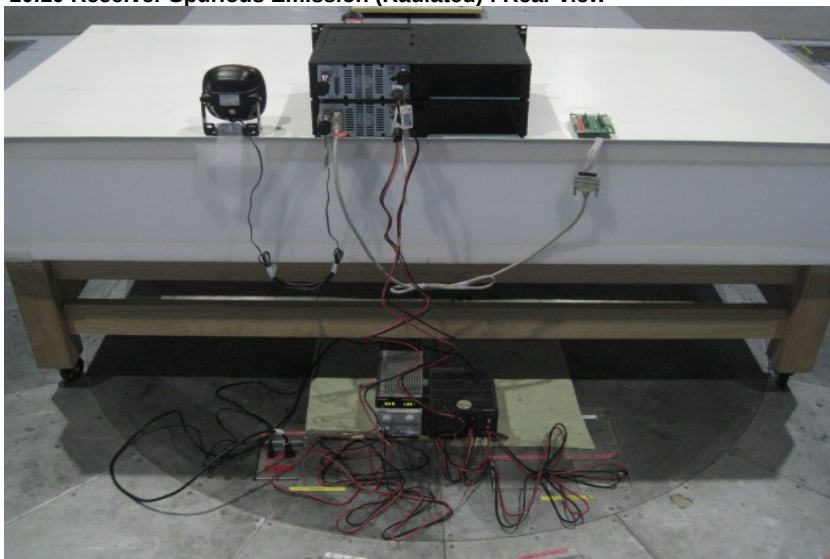
10.10 Receiver Spurious Emission (Radiated) : Rear view
