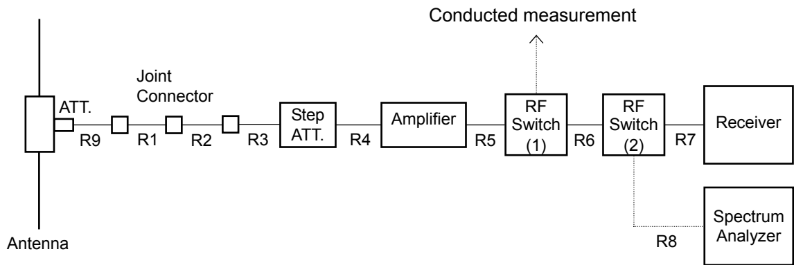
Diagram of the measuring instruments ( 30-1000MHz )
