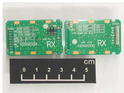
RX PLL VCO Foil Side View
