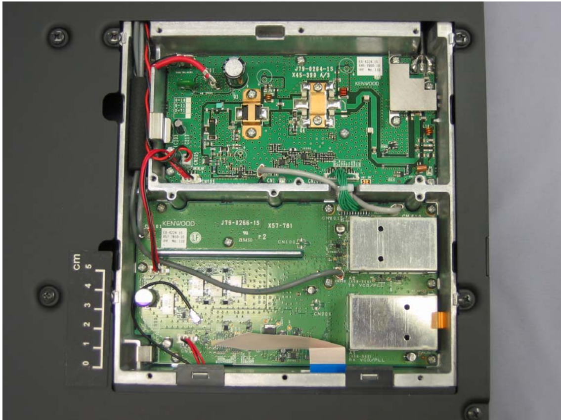
Final Unit / RF Unit
