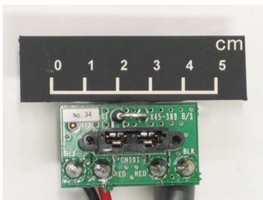
Final A Component Side View
