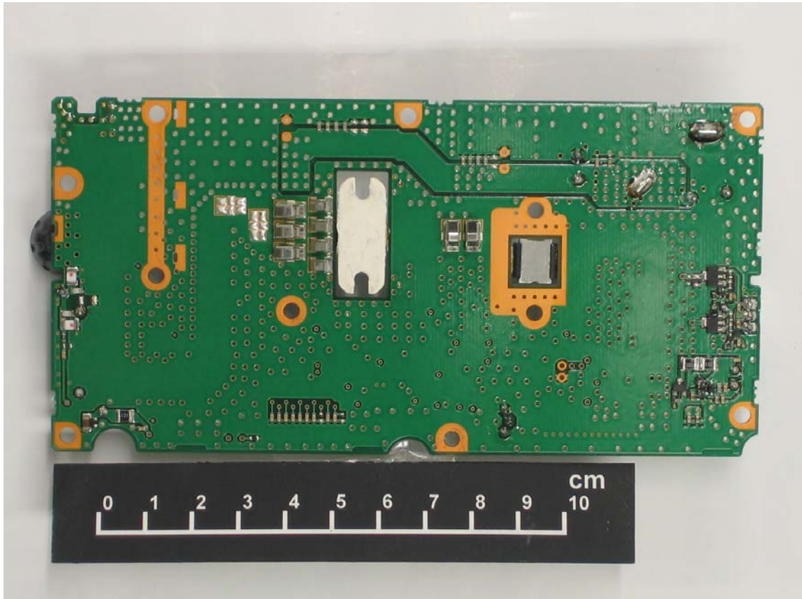
Final Foil Side View
