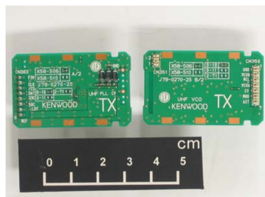
TX PLL VCO Foil Side View
