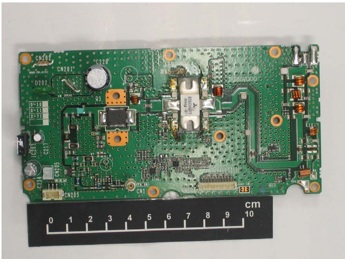
Final Component Side View
