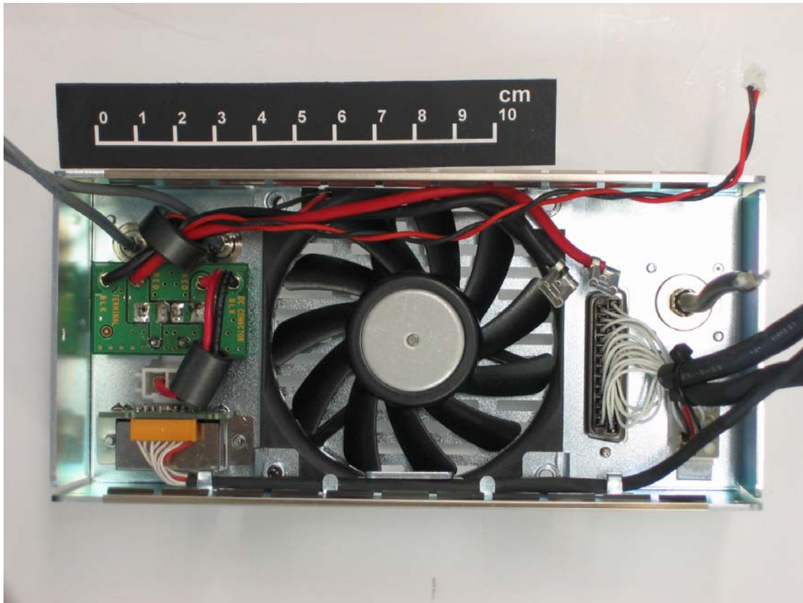
Final A/B Unit
