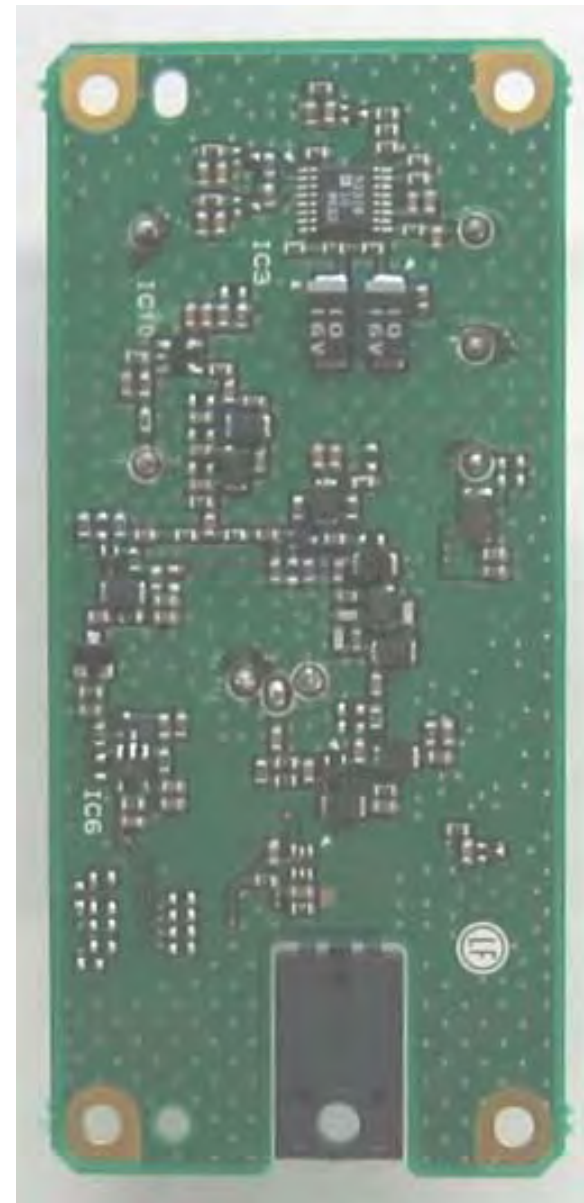
OCXO UNIT Foil Side View
