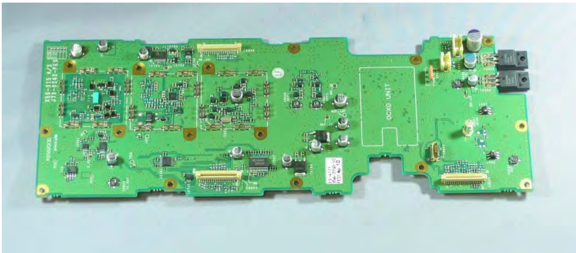
TX Component Side View
