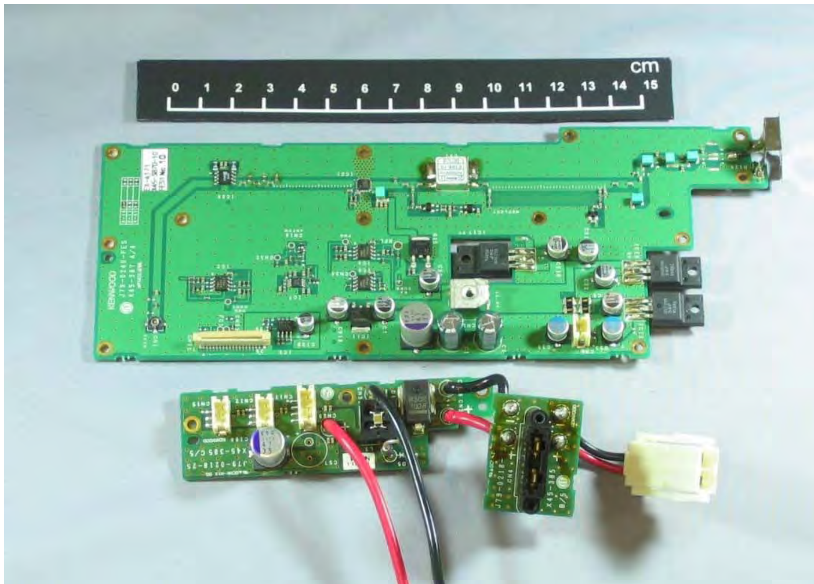
Final Component Side View
