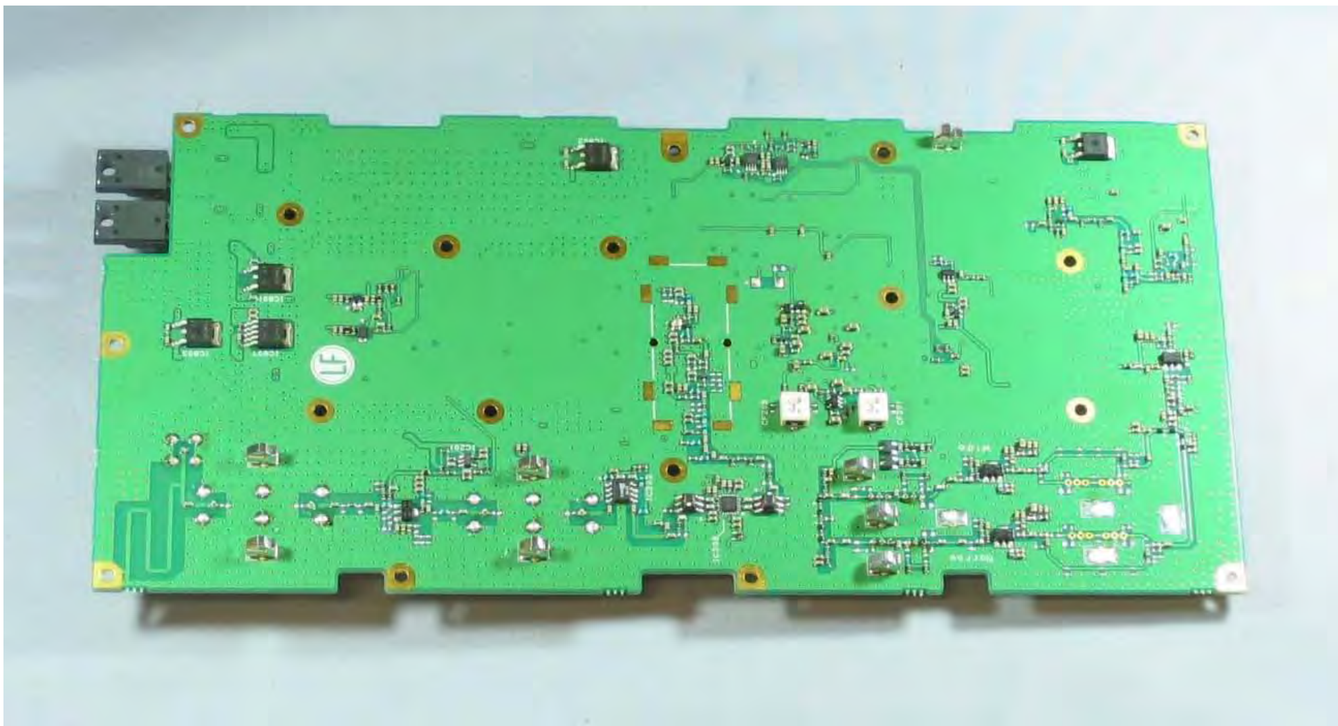
RX Foil Side View
