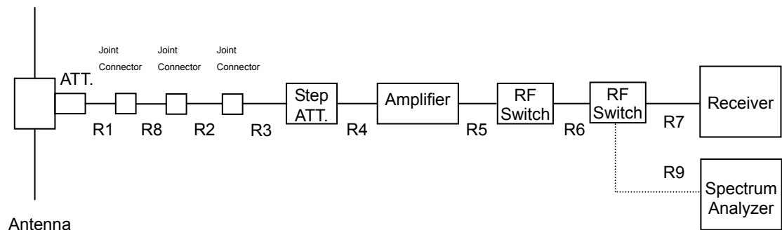
Diagram of the measuring instruments (Above 1000 MHz)
