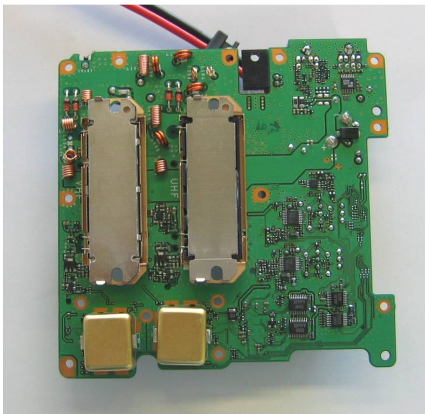
TXRX Unit Foil Side View
