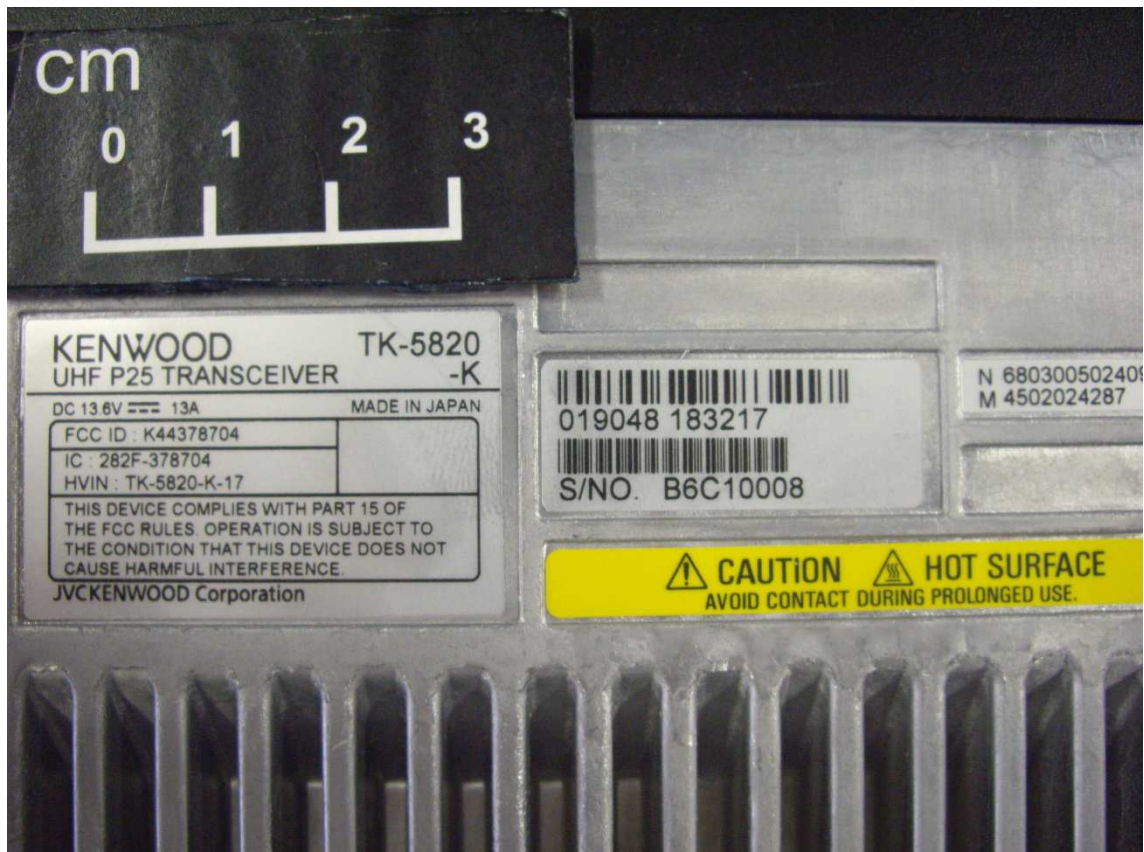
MODEL NAME PLATE LABEL (TK-5820-K)
