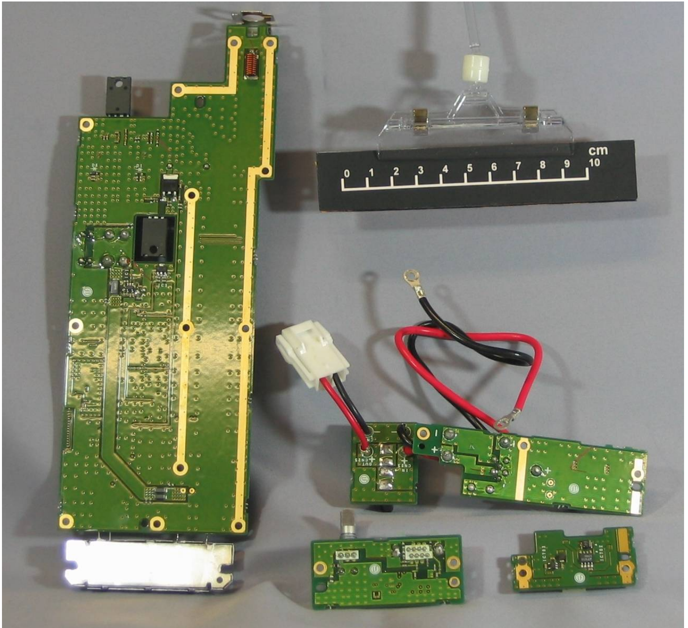
Final Foil Side View
