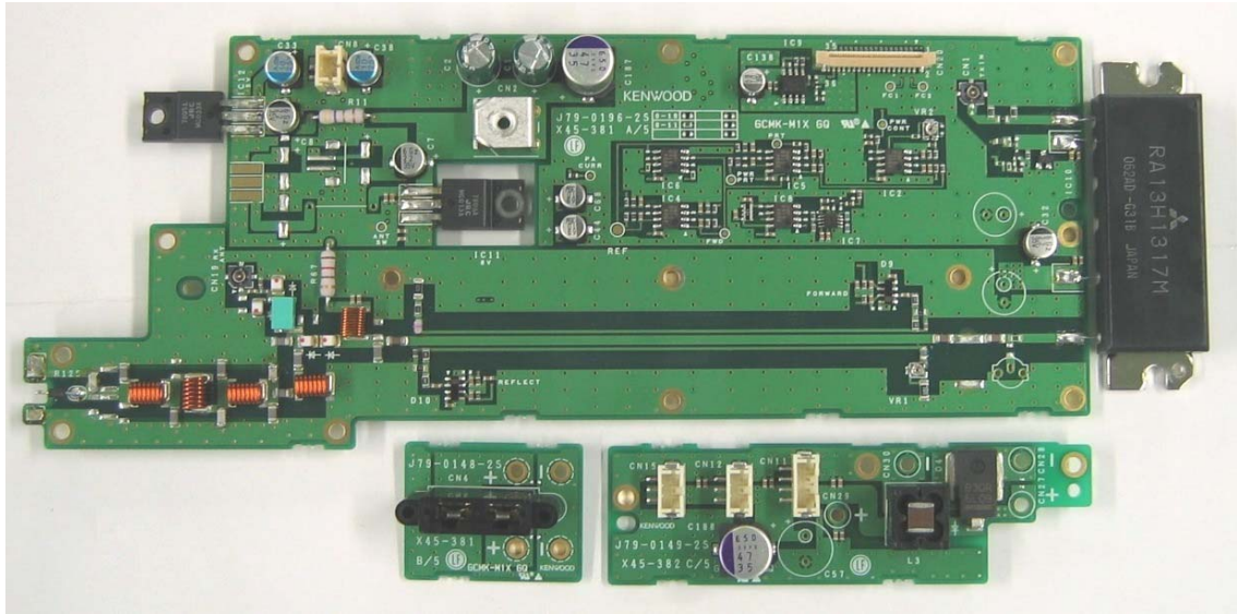
Final Component Side View
