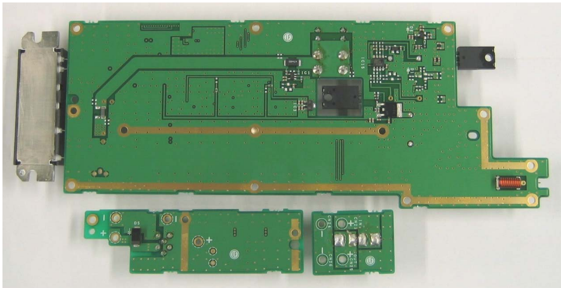
Final Foil Side View
