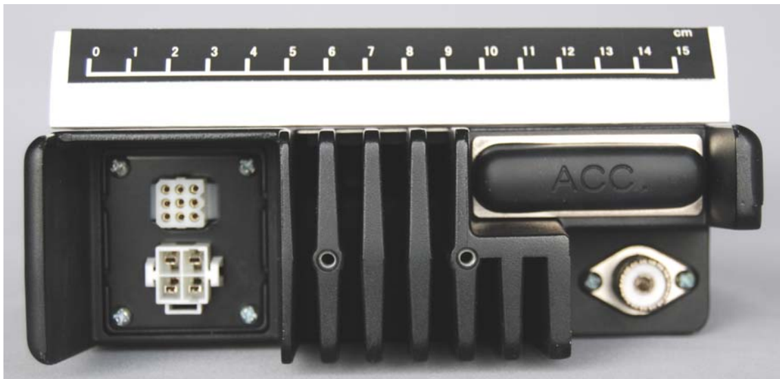
Rear View
