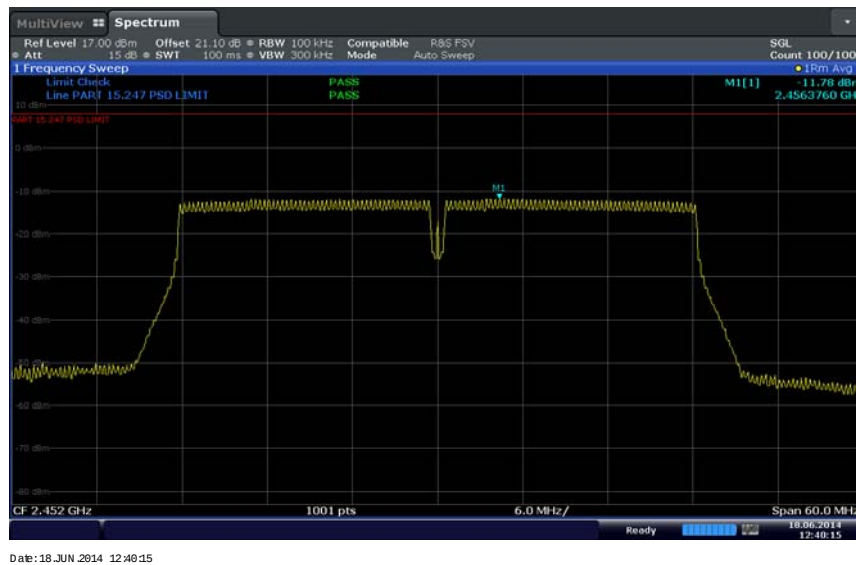
802.11n HT40 Worst Case Channel
