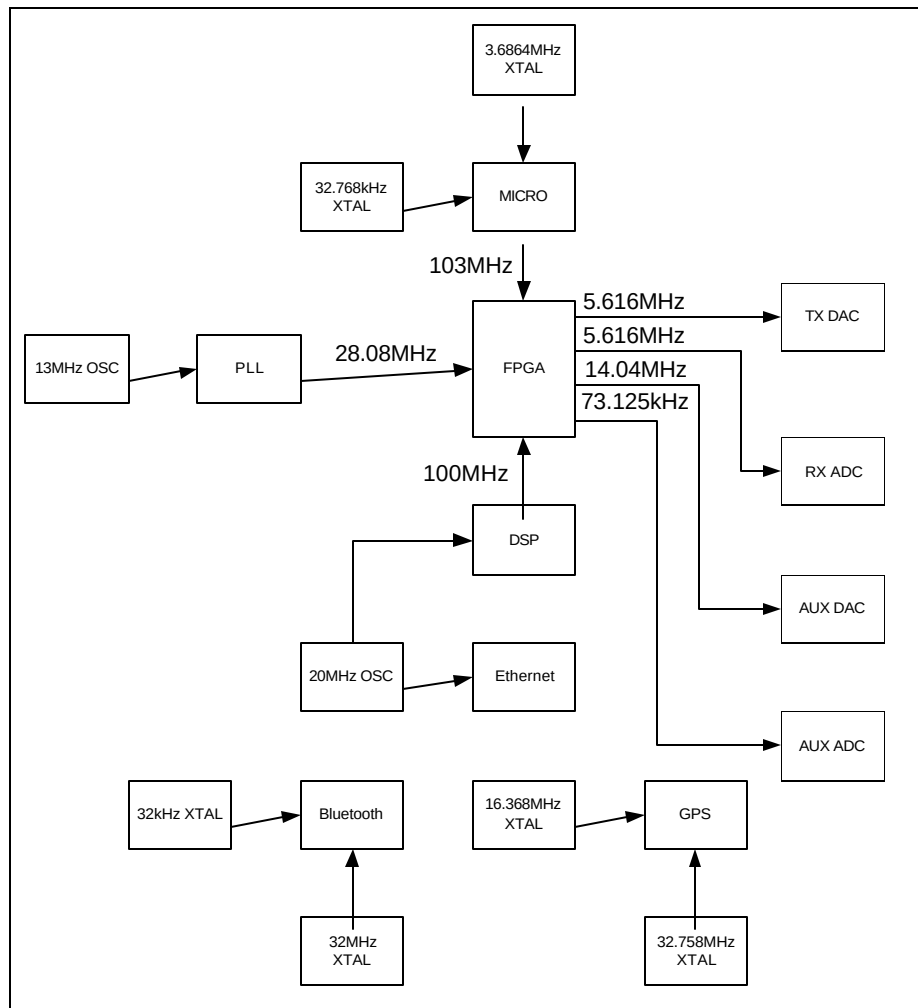
Figure 2. Clock Diagram
