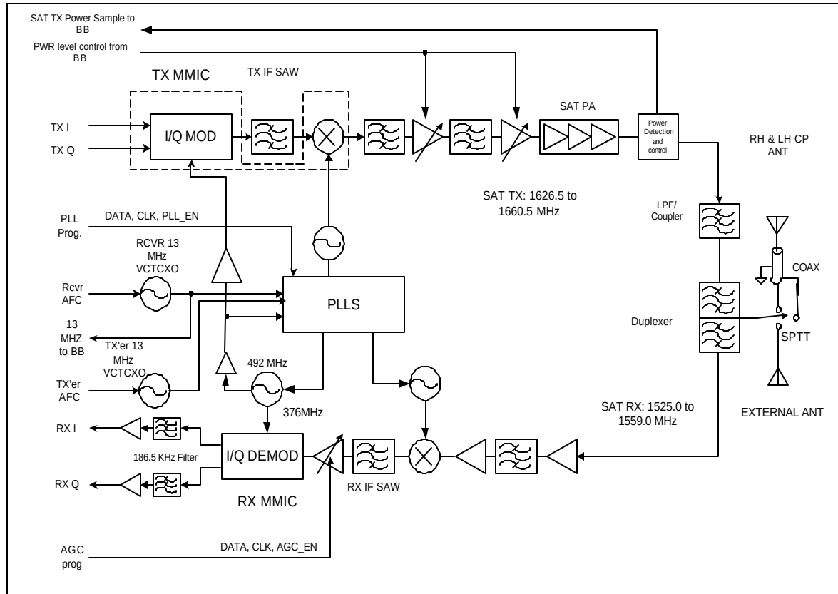
Figure 1. RF Block Diagram
