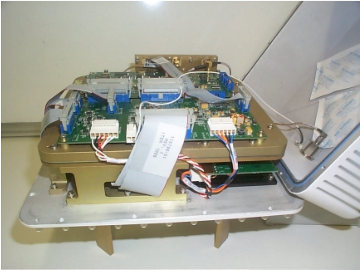
Figure 3: Open ODU SUB photo 3
