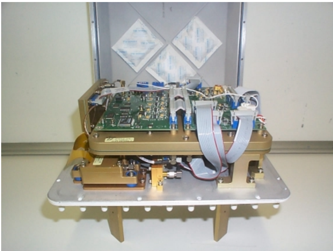
Figure 2: Open ODU SUB photo 2
