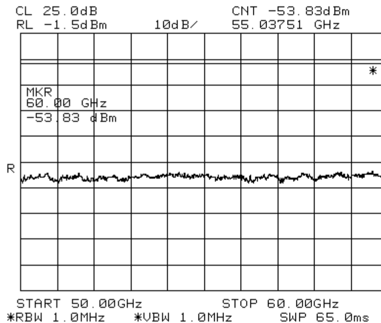
Figure 49 Radiated Emissions in 50-60GHz, VP, for transmitting 18dBm QPSK on Channel 14A4
