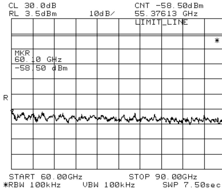
Figure 27 Conducted Emissions in 60-90GHz, for transmitting 18dBm QPSK on Channel 8A1
