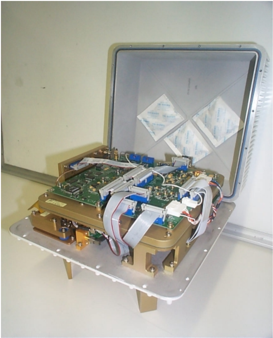
Figure 3 ODU HUB – Open cover
