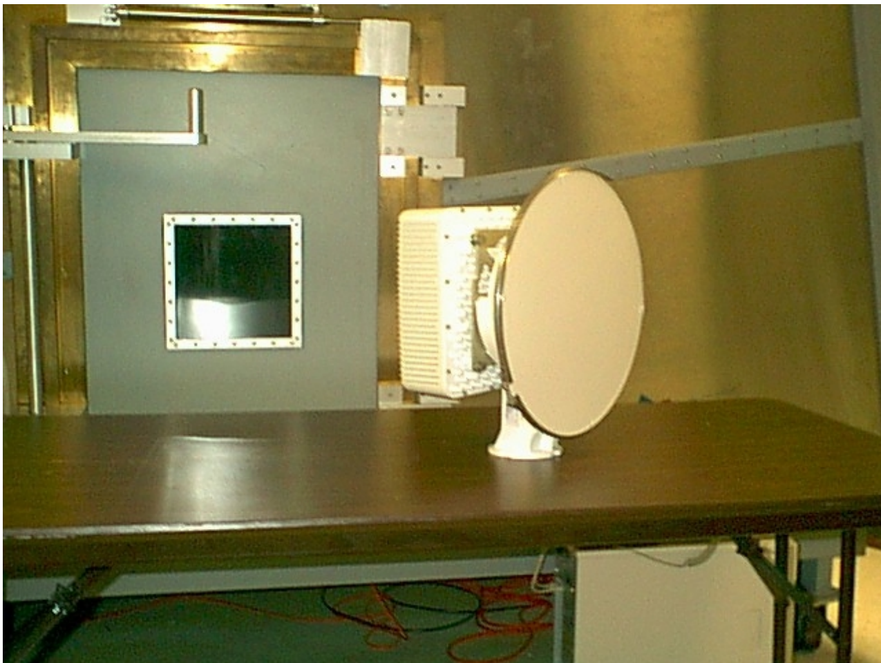
Figure 2 ODU and Antenna - Front View
