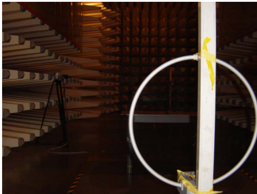
Set-up for Radiation Emission (Transceiver) – Loop Antenna
