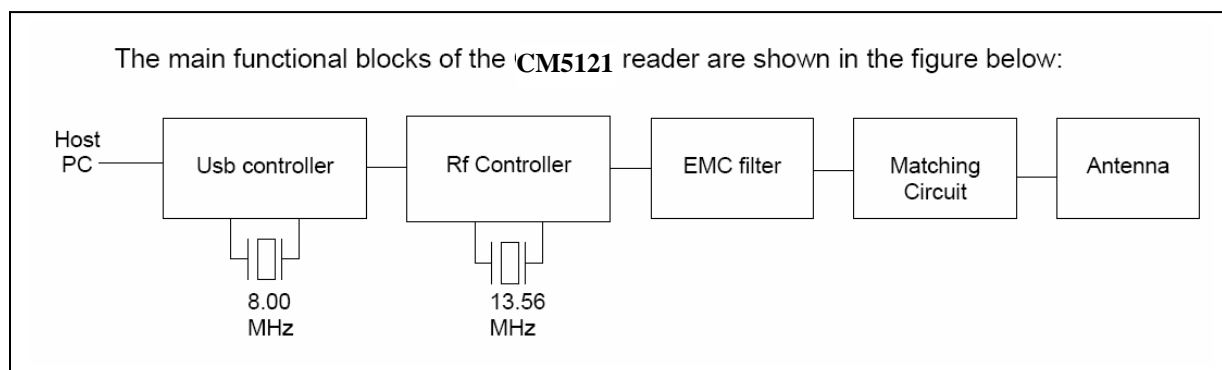
Figure 1: CardMan 5121 block diagram
