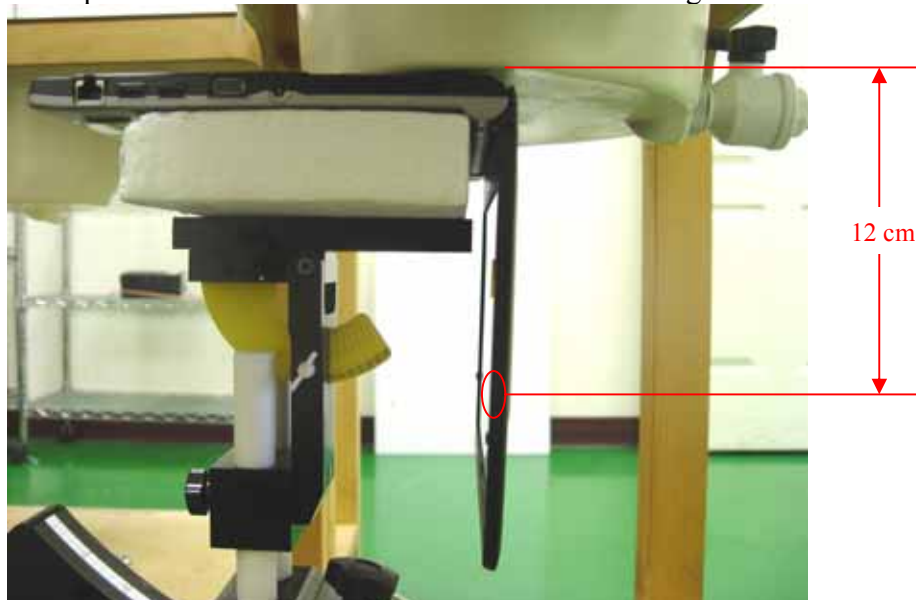
Fig. 9.1 Notebook Bottom Touch
