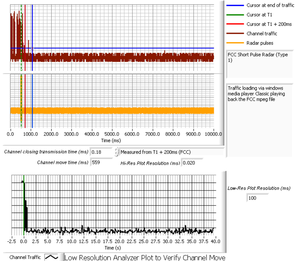
Figure 3 Channel Closing
