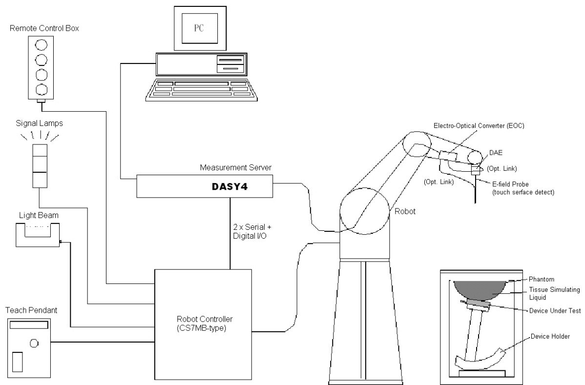
Fig. 5.1 DASY4 System
