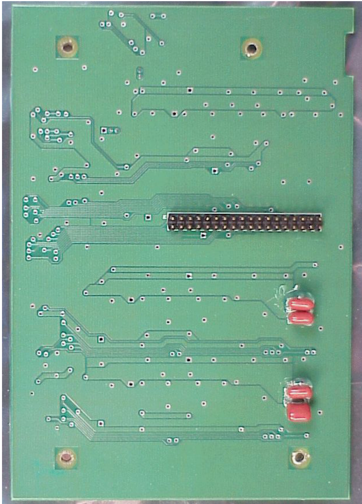
PT-200/PT-210/PT-210M Single-Supply Processor – Bottom Side
