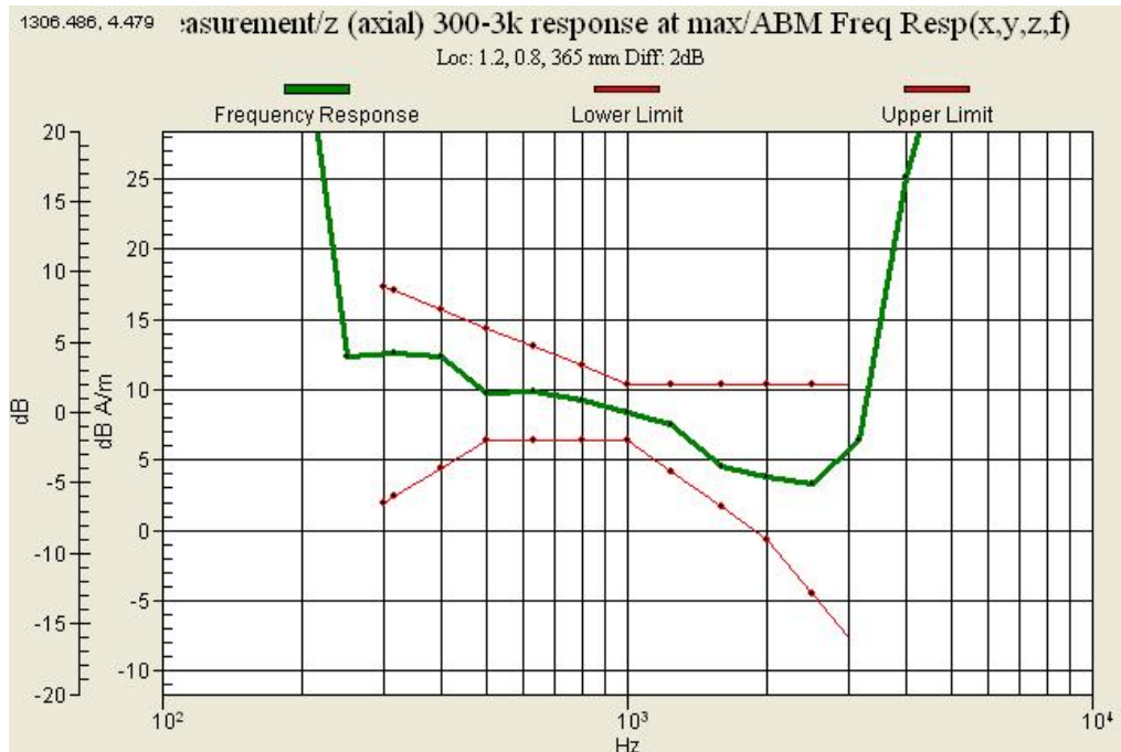
Graph 6 : PCS 1900 (CH 1175) Frequency Response Slide down
