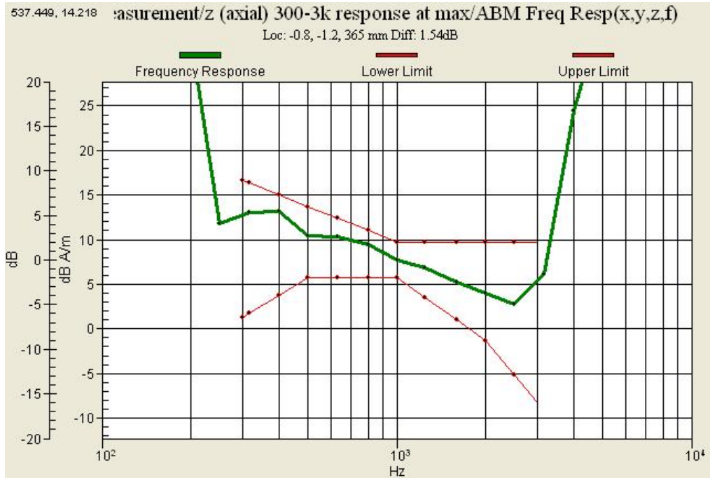
Graph 1 : CDMA 800 (CH 1013) Frequency Response Slide down
