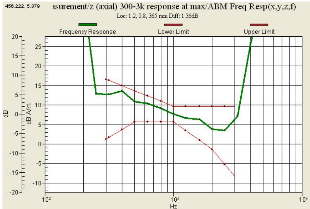
Graph 3 : CDMA 800 (CH 777) Frequency Response Slide down
