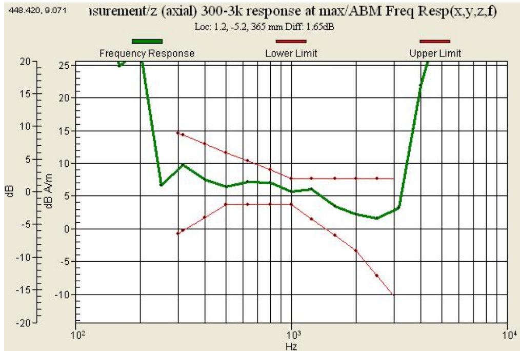
Graph 9 : CDMA 800 (CH 777) Frequency Response Slide up
