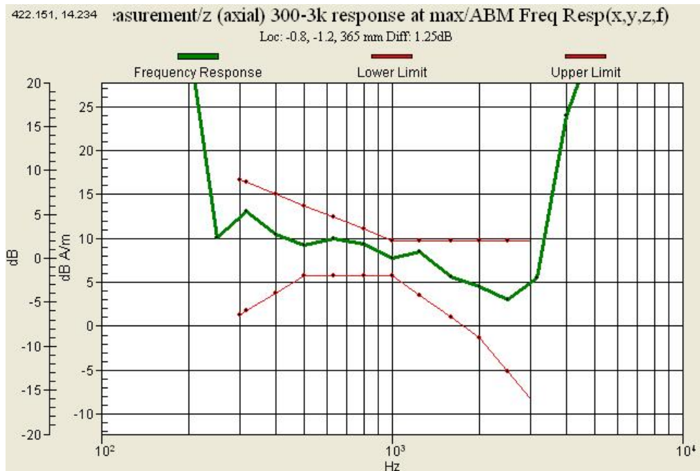
Graph 10 : PCS 1900 (CH 25) Frequency Response Slide up
