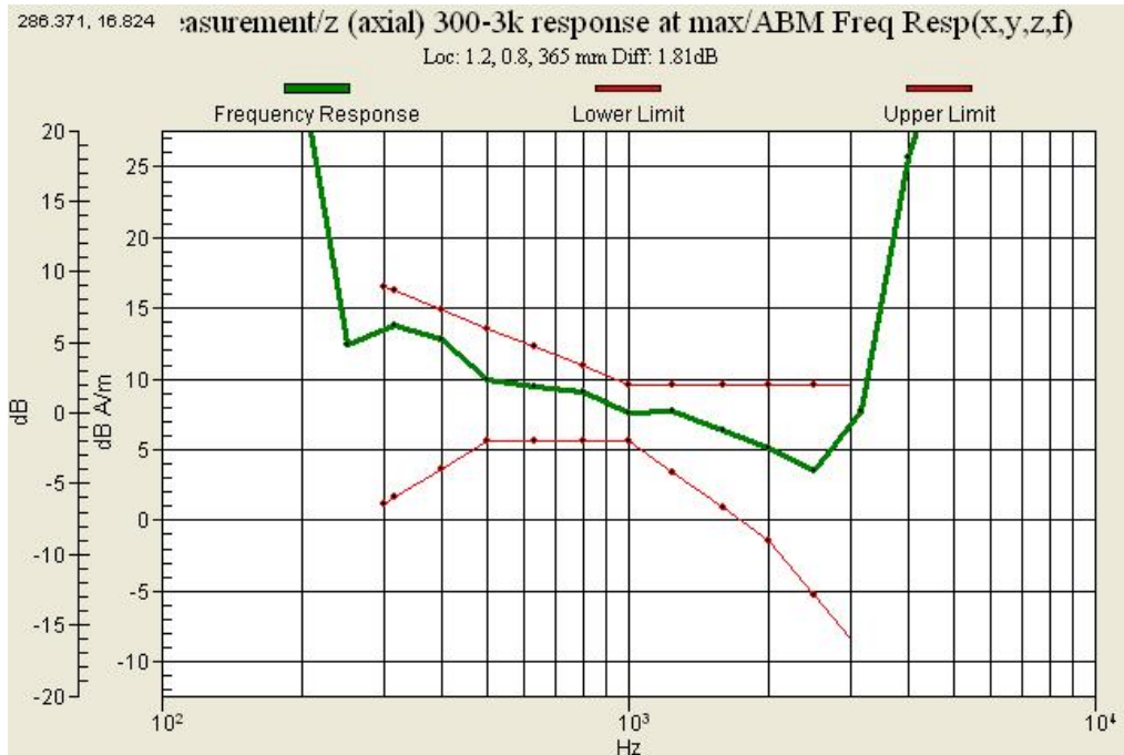
Graph 2 : CDMA 800 (CH 384) Frequency Response Slide down
