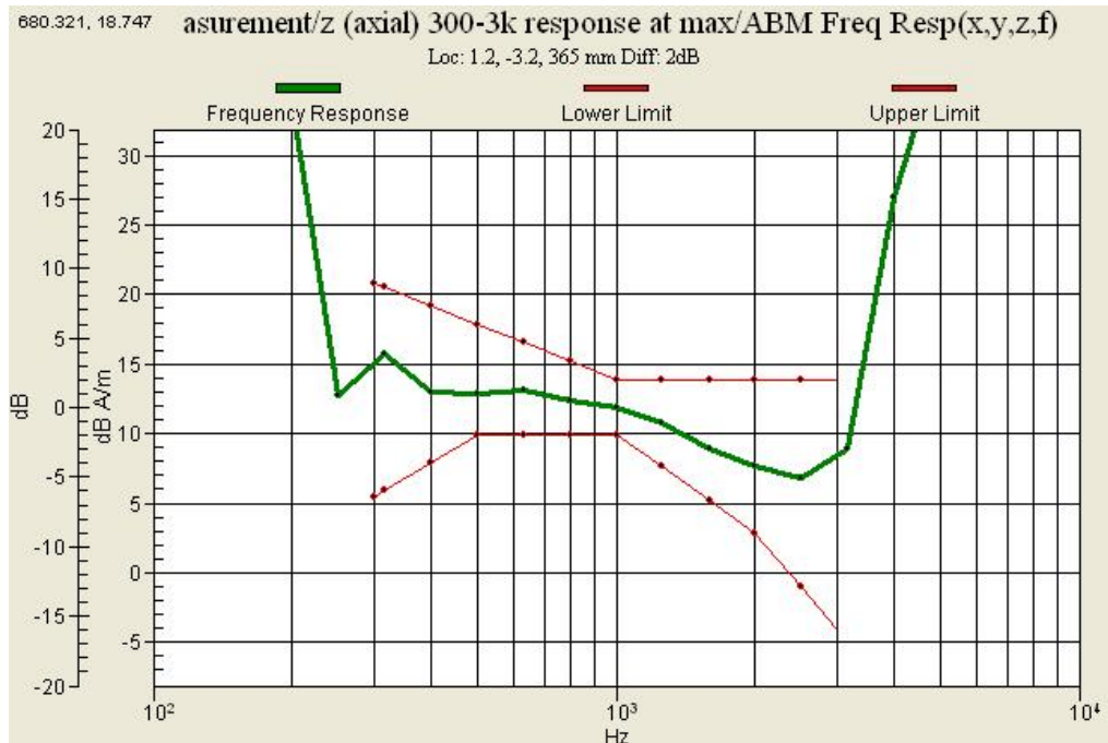
Graph 12 : PCS 1900 (CH 1175) Frequency Response Slide up
