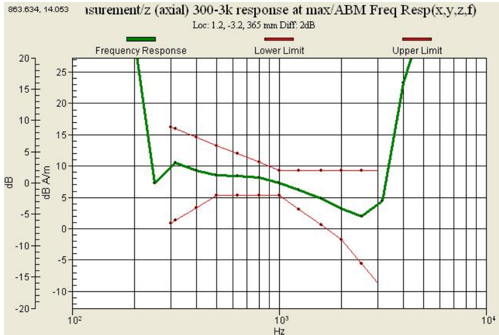
Graph 11 : PCS 1900 (CH 600) Frequency Response Slide up
