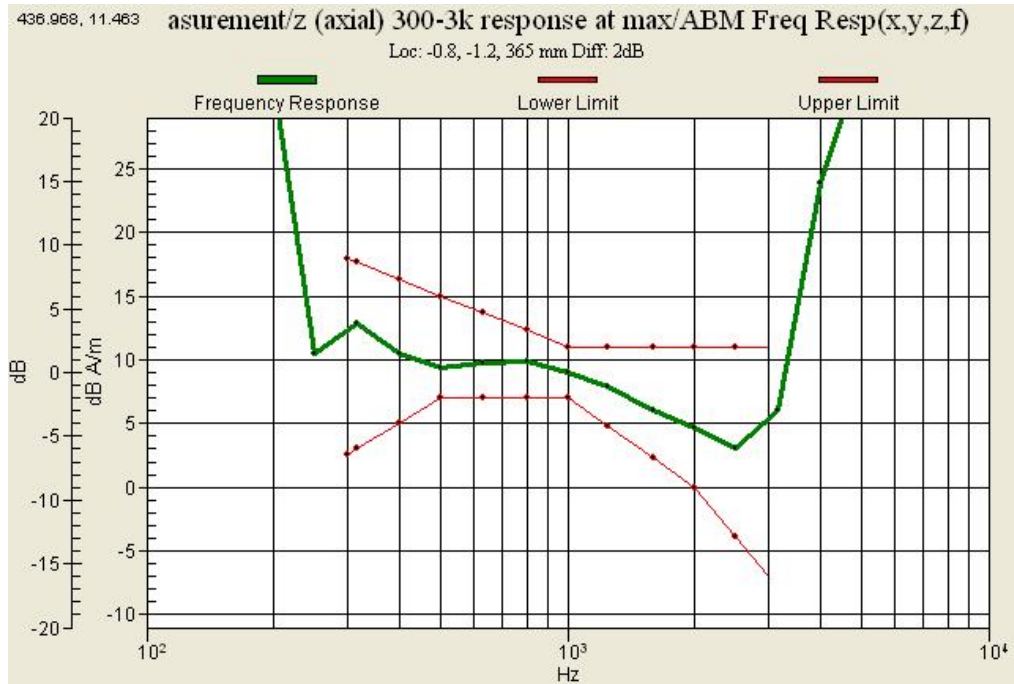
Graph 7 : CDMA 800 (CH 1013) Frequency Response Slide up
