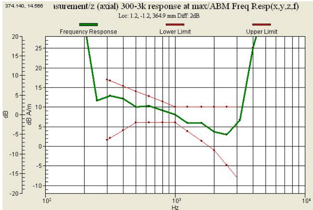
Graph 5 : PCS 1900 (CH 600) Frequency Response Slide down
