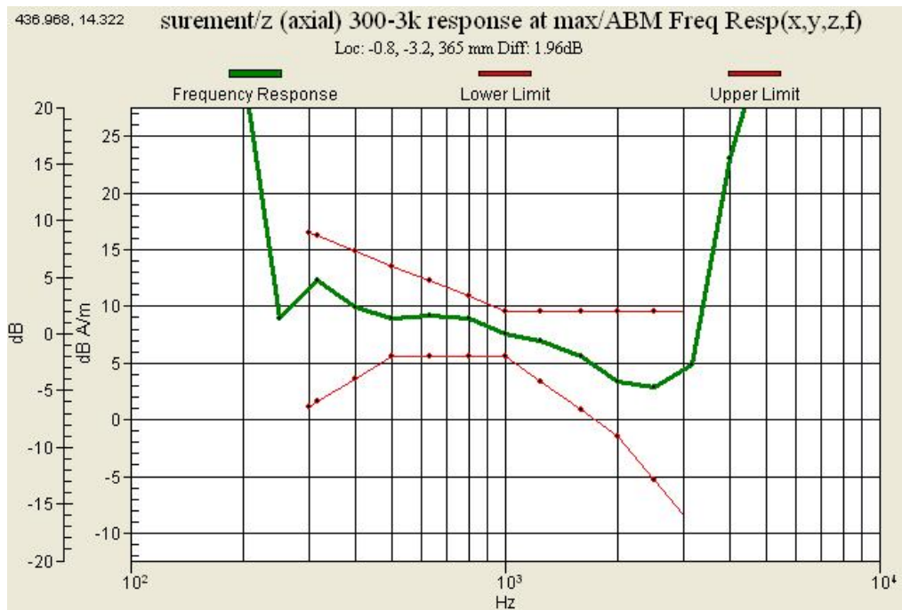
Graph 8 : CDMA 800 (CH 384) Frequency Response Slide up
