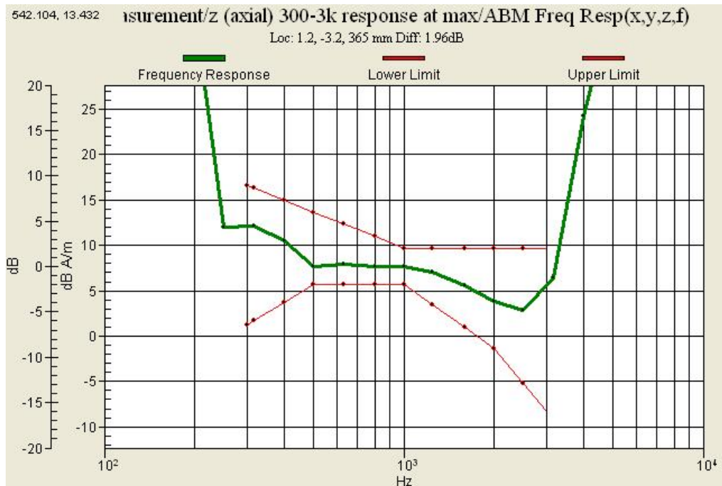
Graph 4 : PCS 1900 (CH 25) Frequency Response Slide down
