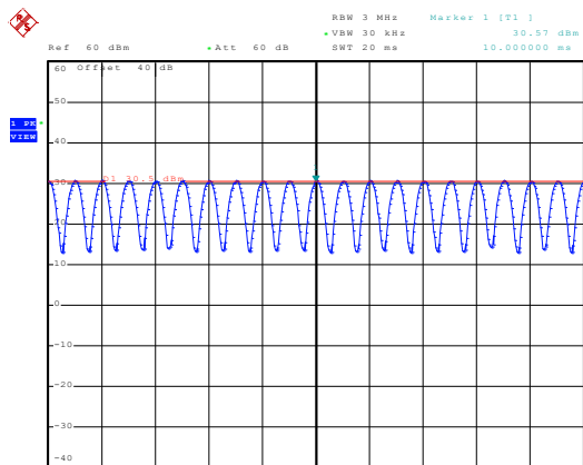
1880MHz - 80% AM
