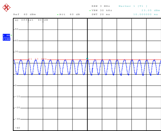
835MHz - 80% AM
