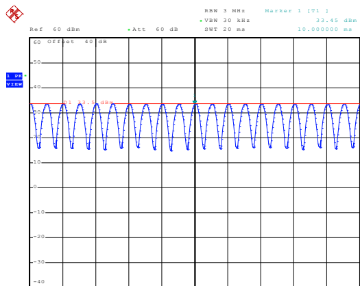
835MHz - 80% AM
