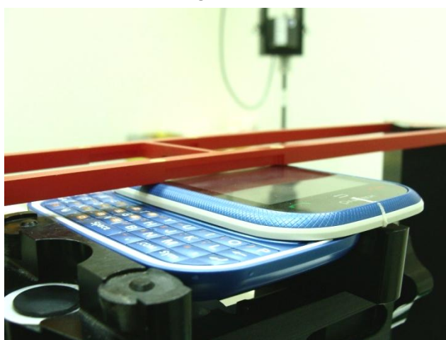
DUT Slide Right - Right Side View
