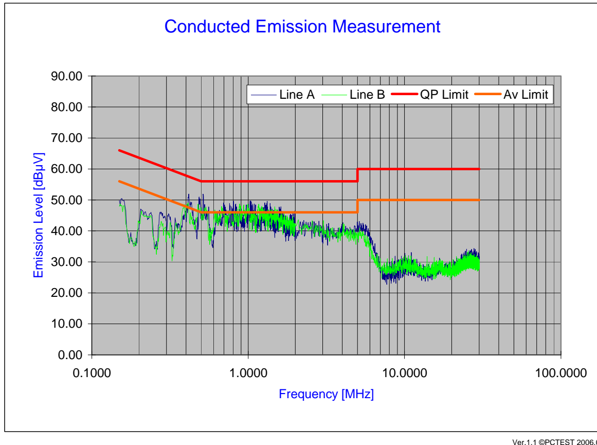
Plot 6-24. Line Conducted Plot with Bluetooth
