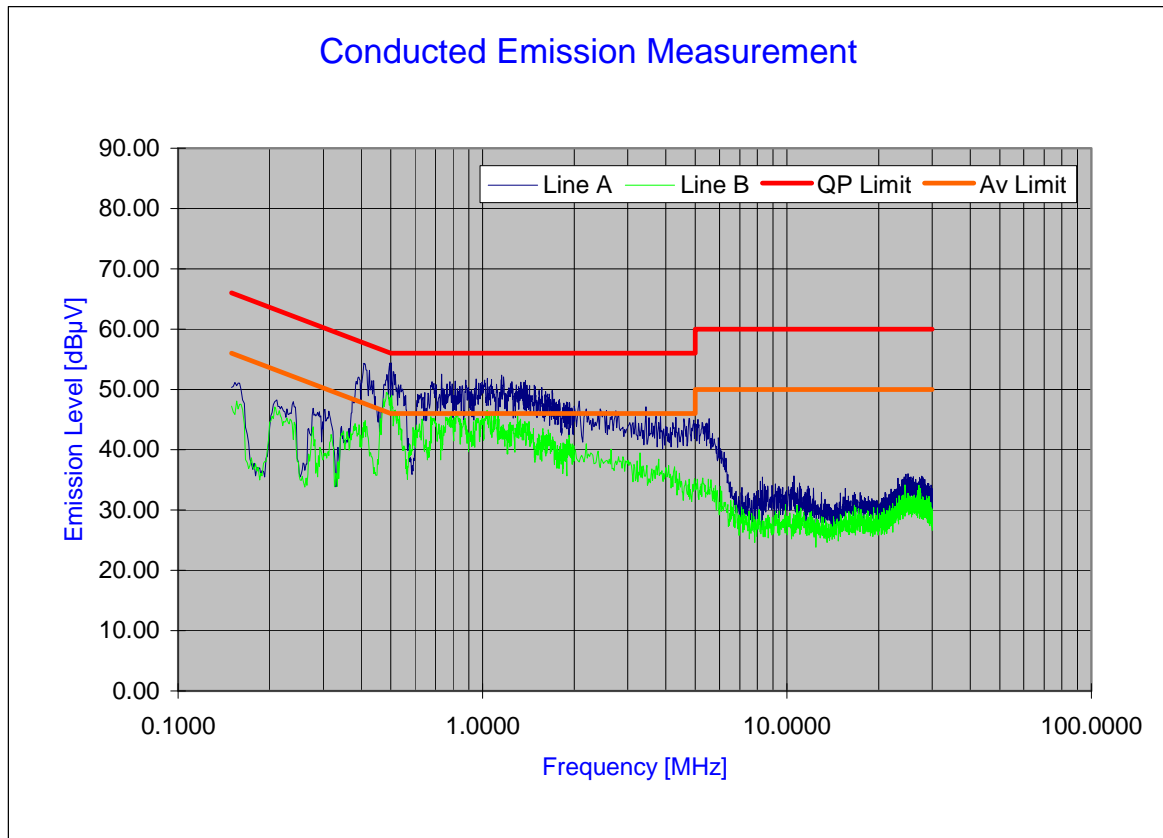
Plot 6-54. Line Conducted Plot with 802.11a
