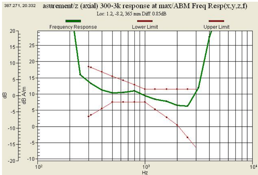
Graph 4 : GSM 1900(CH 512) Frequency Response
