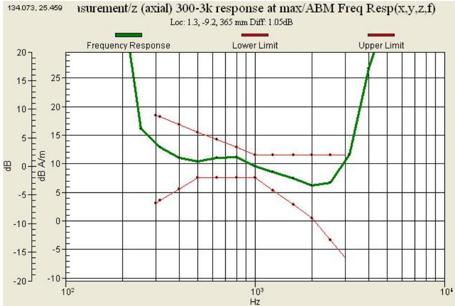
Graph 1 : GSM 850 (CH 128) Frequency Response
