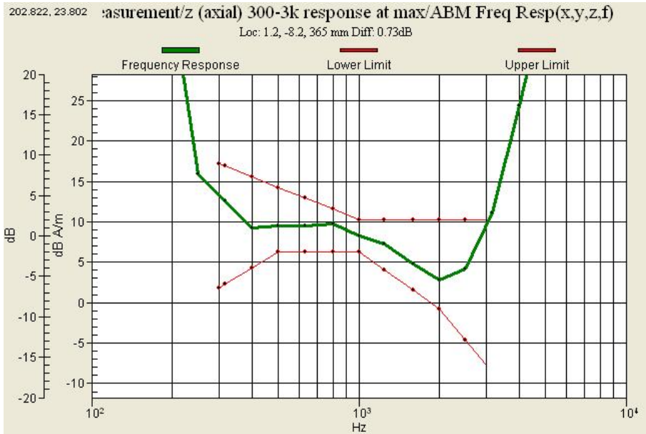
Graph 11 : WCDMA 1900 (CH 9400) Frequency Response
