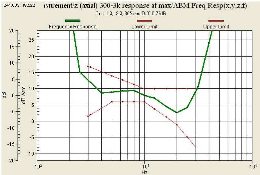
Graph 7 : WCDMA 850 (CH 4132) Frequency Response
