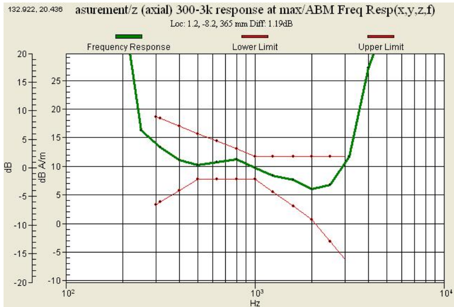
Graph 6 : GSM 1900 (CH 810) Frequency Response
