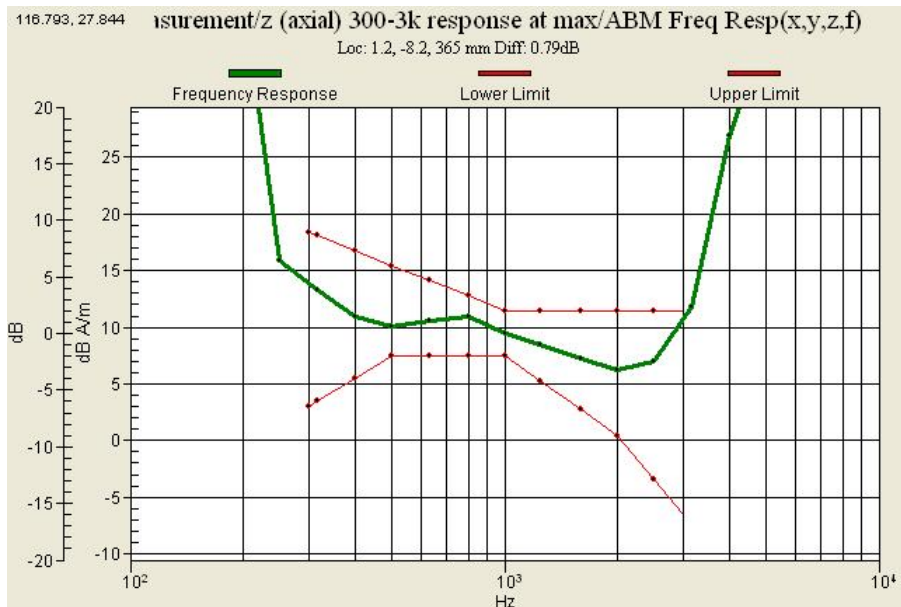
Graph 2 : GSM 850(CH 190) Frequency Response
