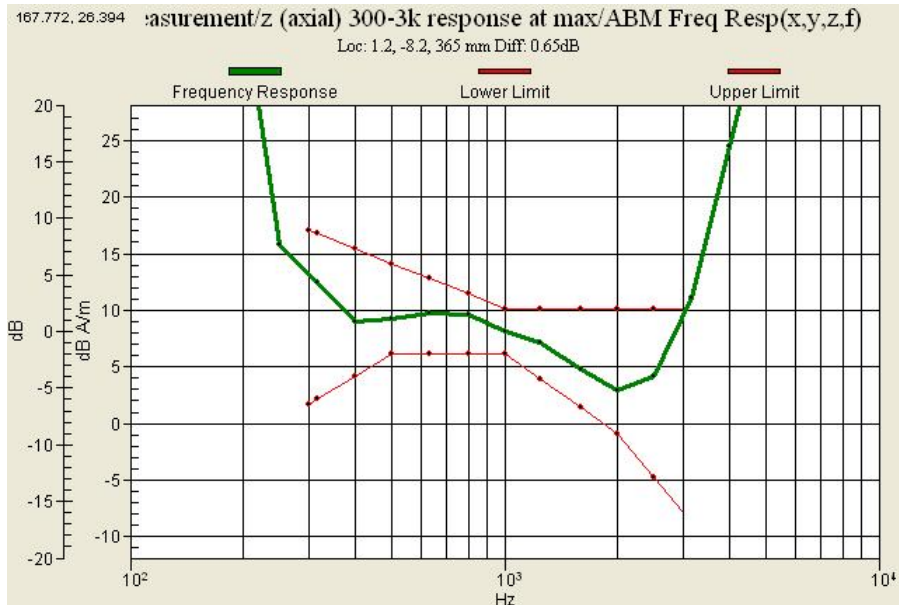
Graph 10 : WCDMA 1900 (CH 9262) Frequency Response
