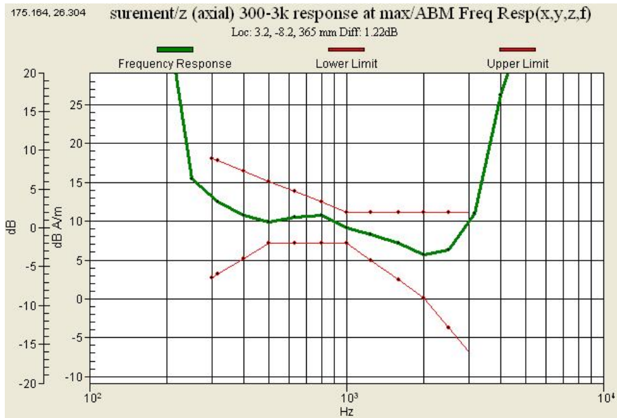
Graph 5 : GSM 1900 (CH 661) Frequency Response
