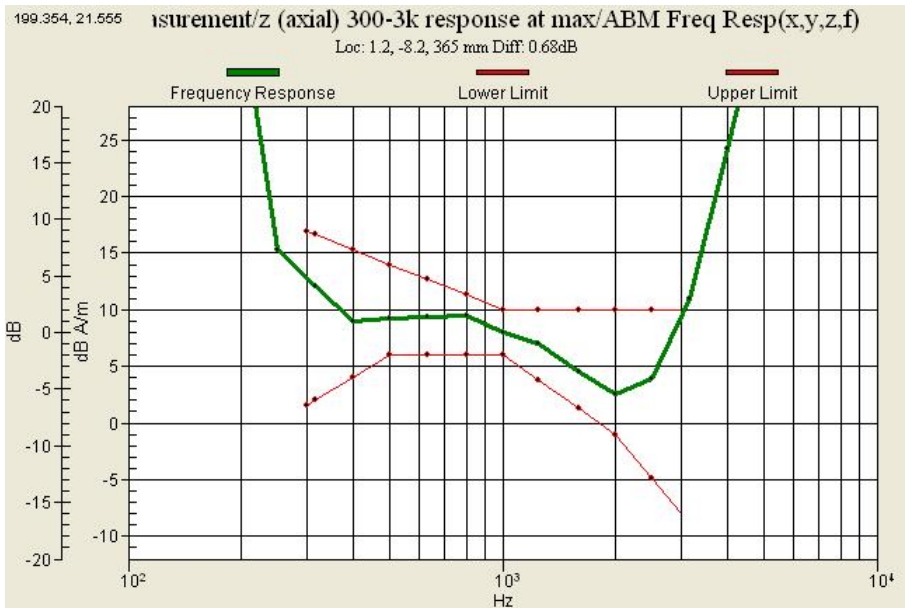
Graph 8 : WCDMA 850(CH 4183) Frequency Response
