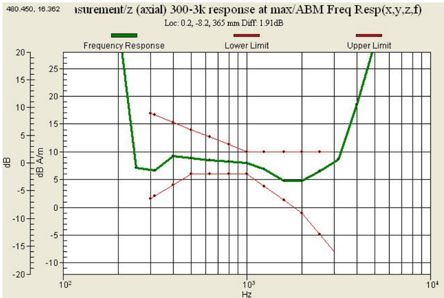
Graph 12 : WCDMA 1900 (CH 9583) Frequency Response
