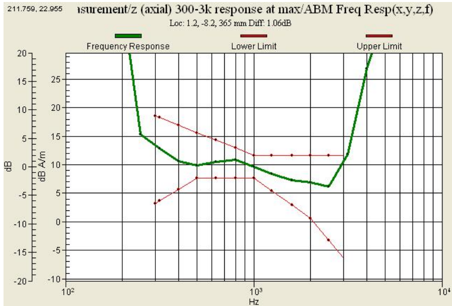
Graph 3 : GSM 850 (CH 251) Frequency Response
