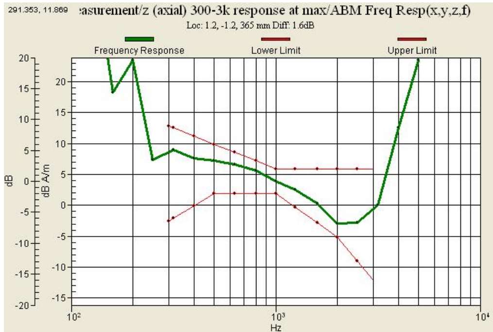
Graph 9 : WCDMA 850 (CH 4233) Frequency Response Slide down
