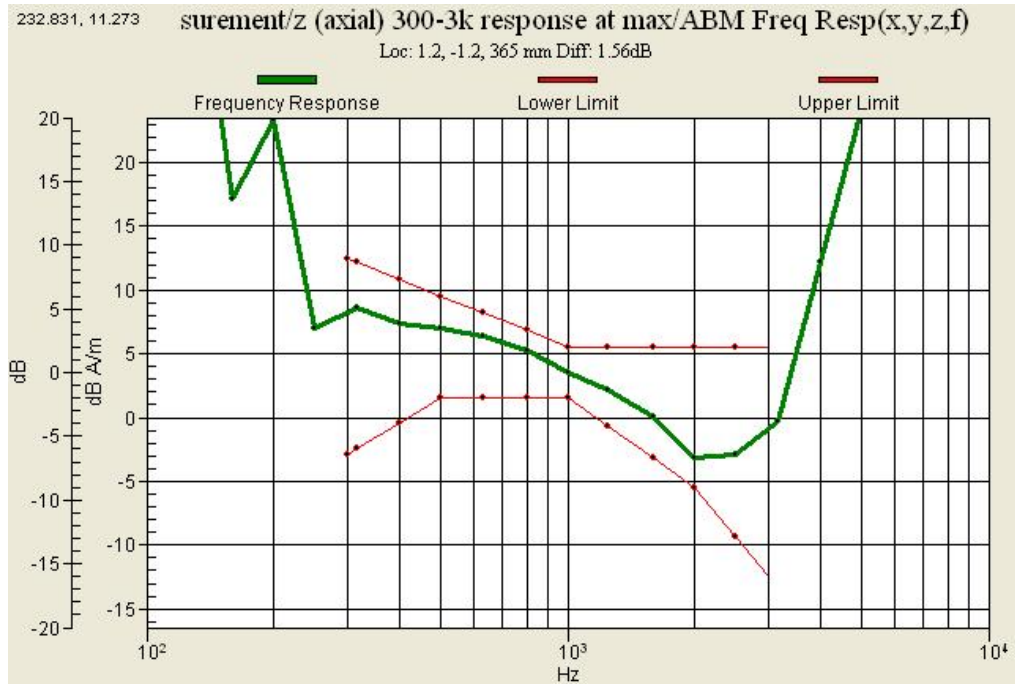
Graph 20 : WCDMA 850(CH 4183) Frequency Response Slide up
