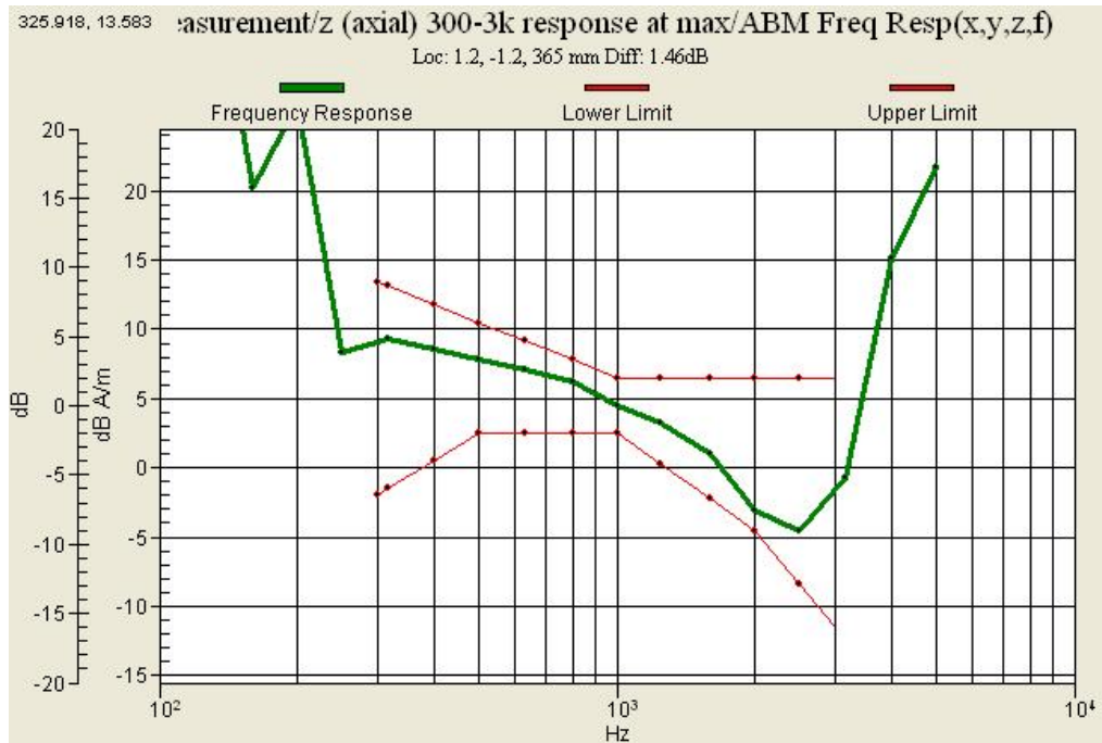
Graph 3 : GSM 850 (CH 251) Frequency Response Slide down
