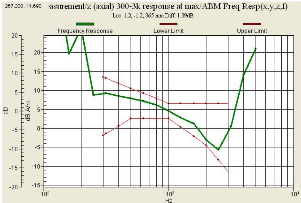
Graph 18 : GSM 1900 (CH 810) Frequency Response Slide up
