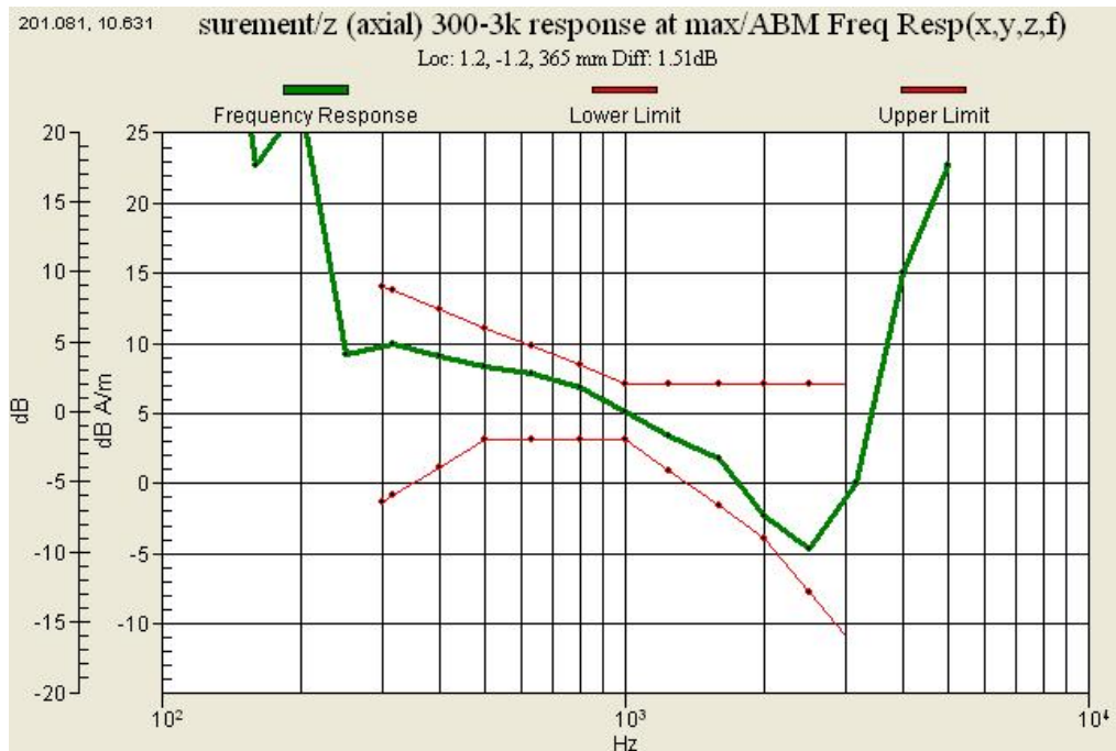
Graph 2 : GSM 850(CH 190) Frequency Response Slide down
