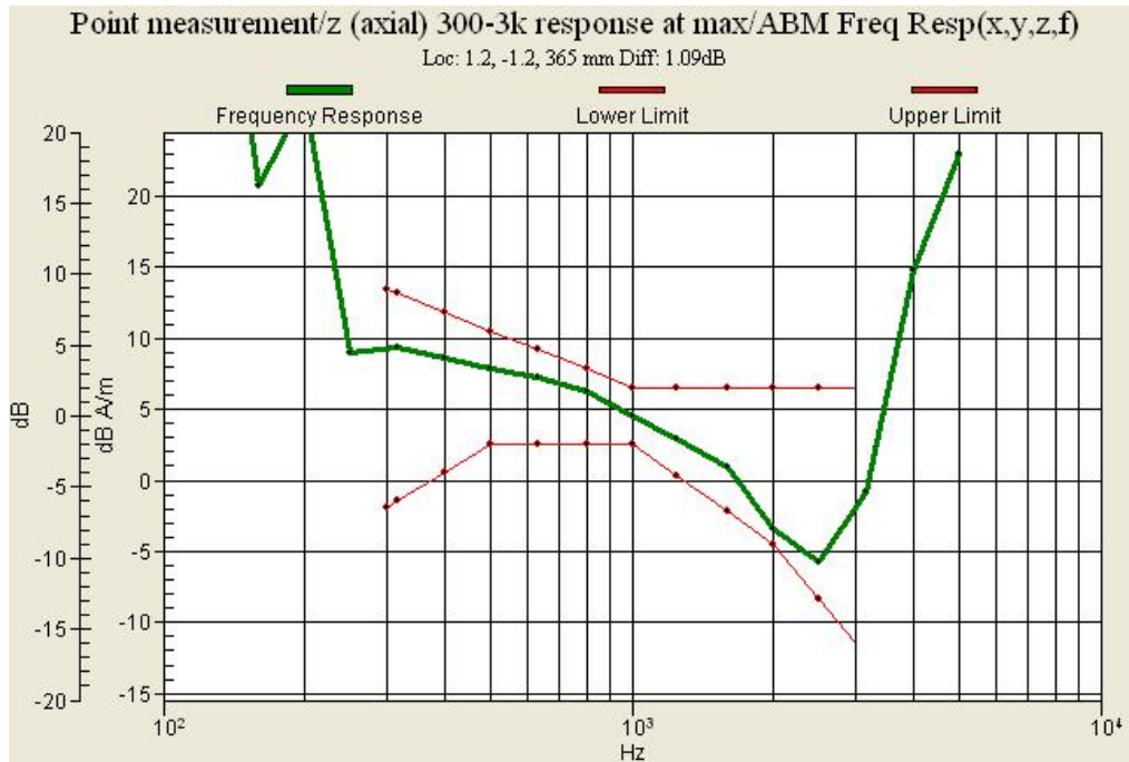
Graph 15 : GSM 850 (CH 251) Frequency Response Slide up
