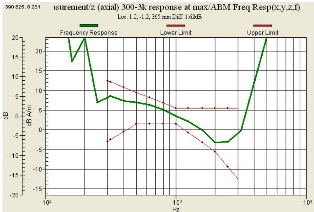
Graph 21 : WCDMA 850 (CH 4233) Frequency Response Slide up
