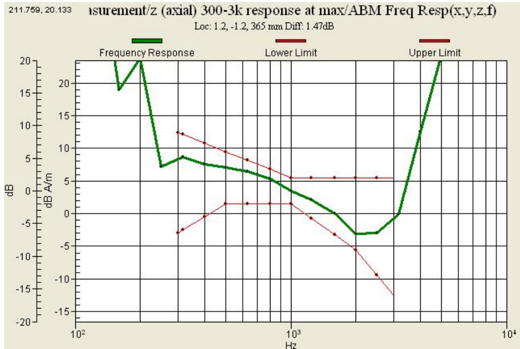
Graph 10 : WCDMA 1900 (CH 9262) Frequency Response Slide down
