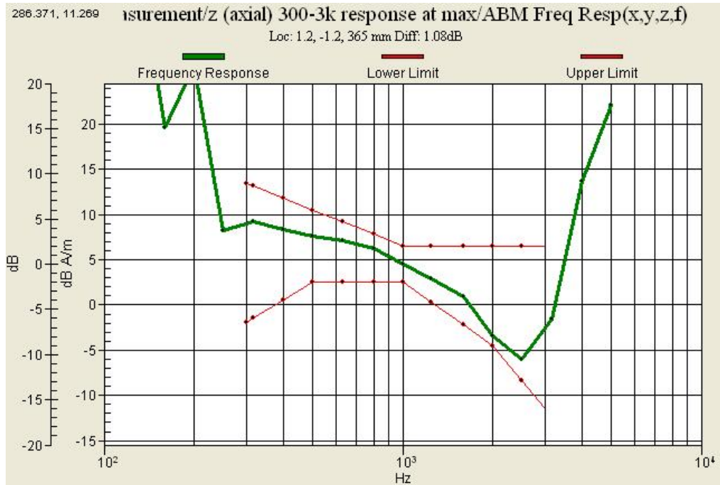
Graph 5 : GSM 1900 (CH 661) Frequency Response Slide down
