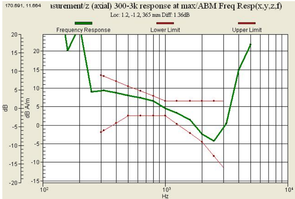
Graph 13 : GSM 850 (CH 128) Frequency Response Slide up
