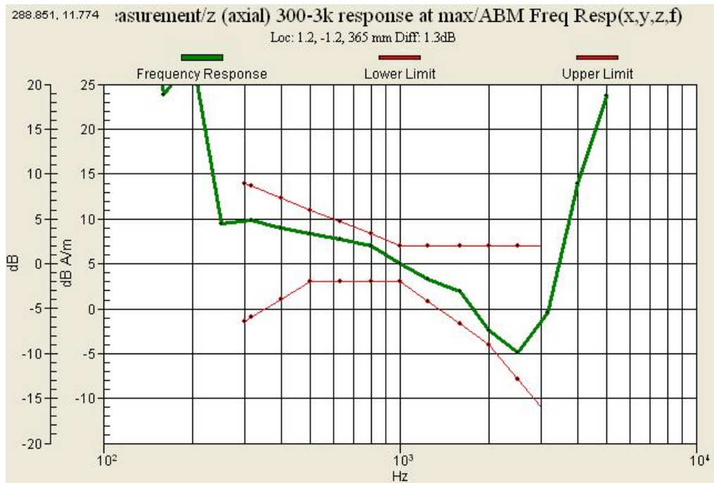
Graph 1 : GSM 850 (CH 128) Frequency Response Slide down
