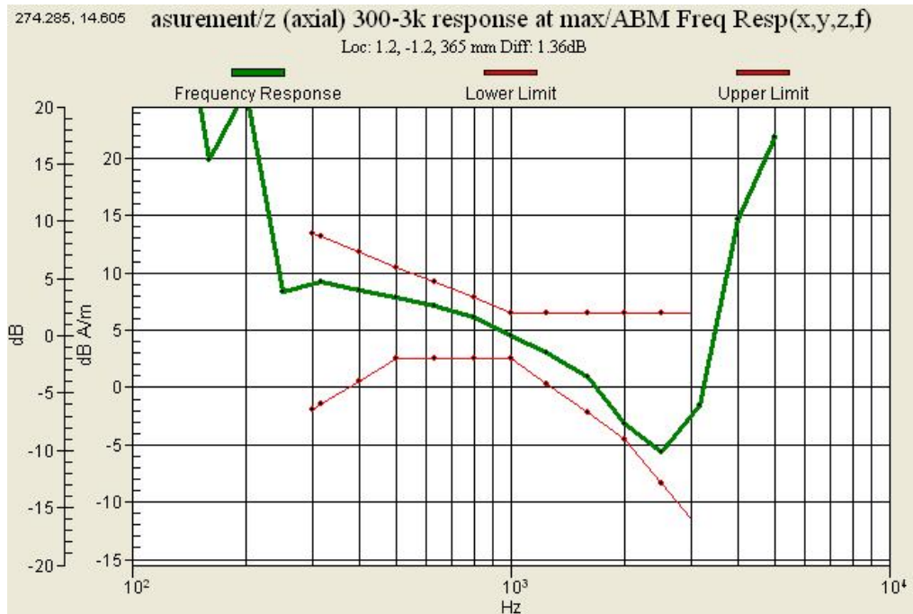
Graph 6 : GSM 1900 (CH 810) Frequency Response Slide down
