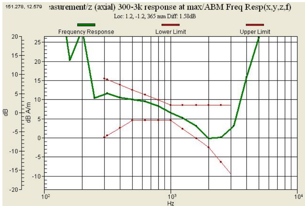
Graph 24 : WCDMA 1900 (CH 9583) Frequency Response Slide up
