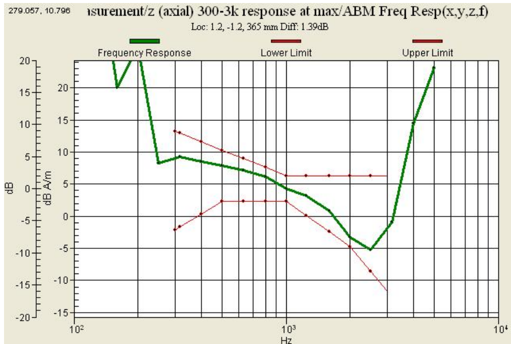
Graph 4 : GSM 1900(CH 512) Frequency Response Slide down
