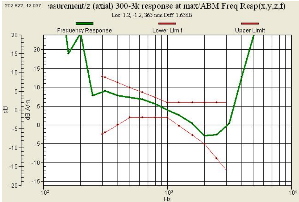
Graph 8 : WCDMA 850(CH 4183) Frequency Response Slide down
