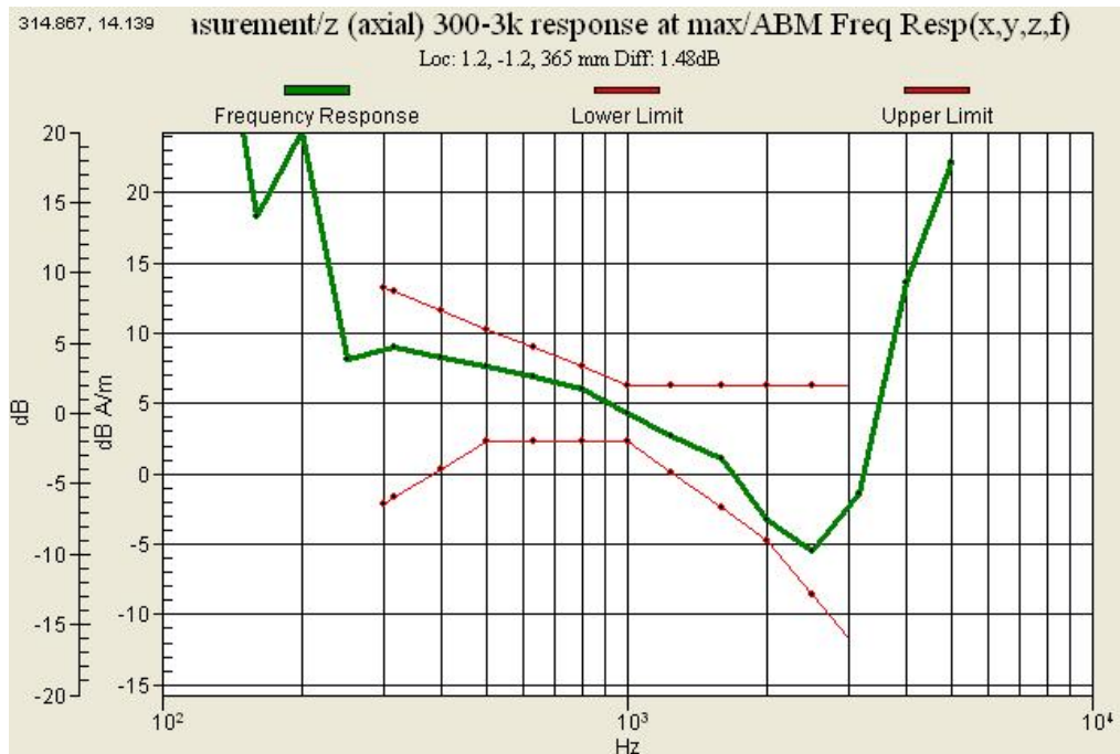
Graph 16 : GSM 1900(CH 512) Frequency Response Slide up
