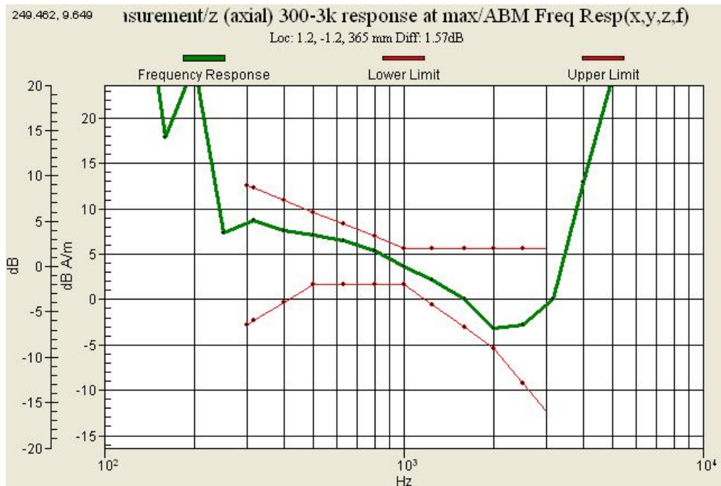
Graph 22 : WCDMA 1900 (CH 9262) Frequency Response Slide up
