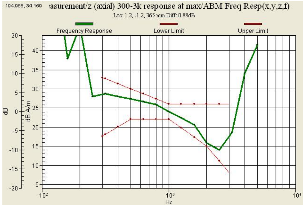
Graph 17 : GSM 1900 (CH 661) Frequency Response Slide up
