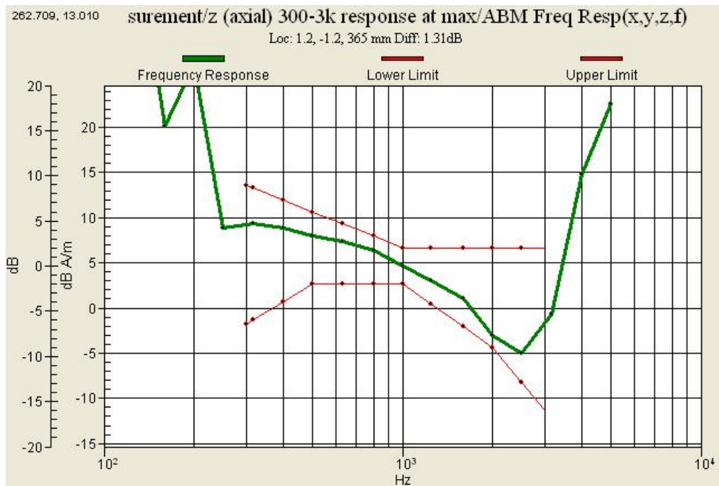
Graph 14 : GSM 850(CH 190) Frequency Response Slide up
