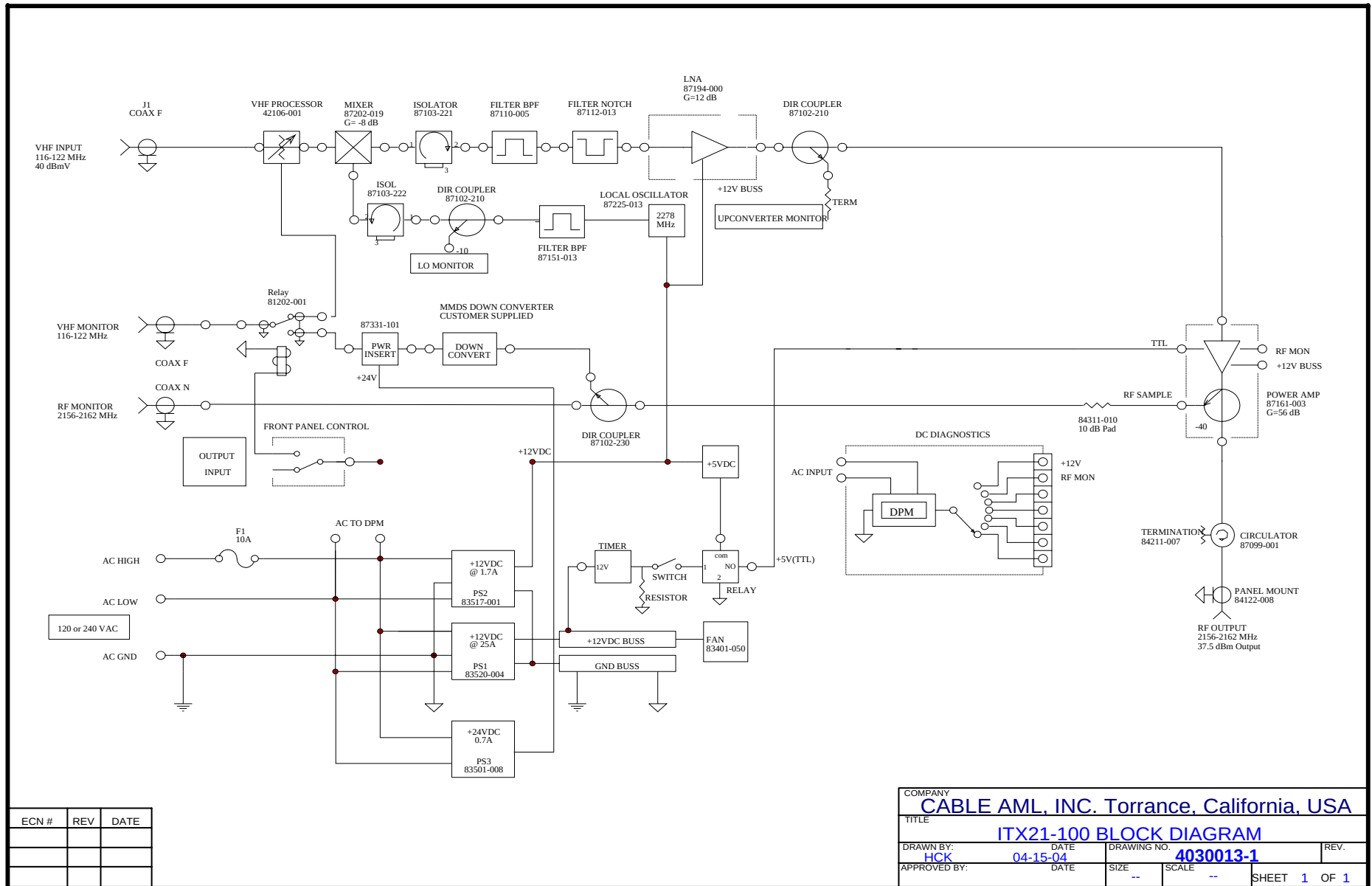
Figure 10. ITX21-100 Transmitter Schematic.
