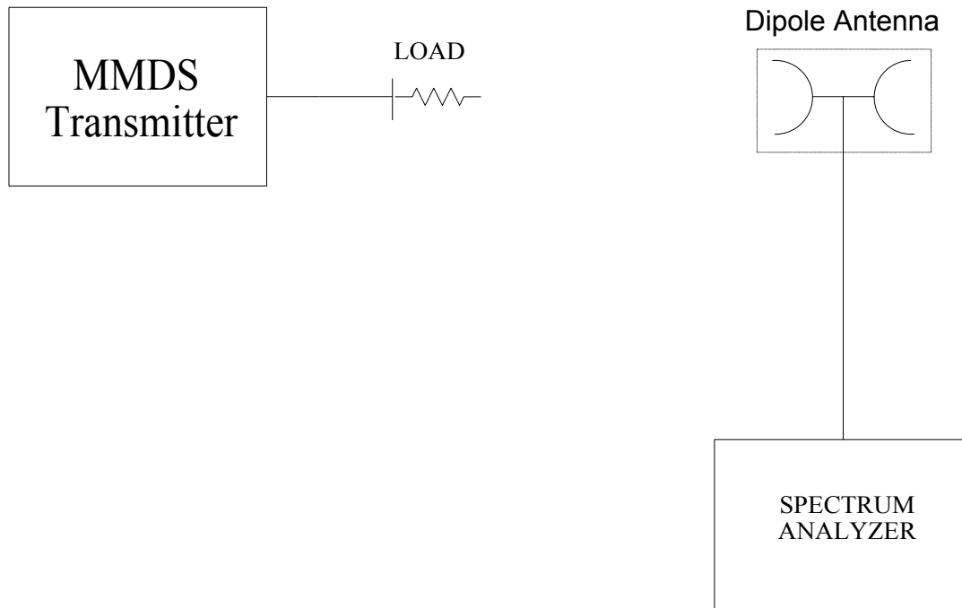
Figure 17. Radiated Emissions Measurement Set-up.
