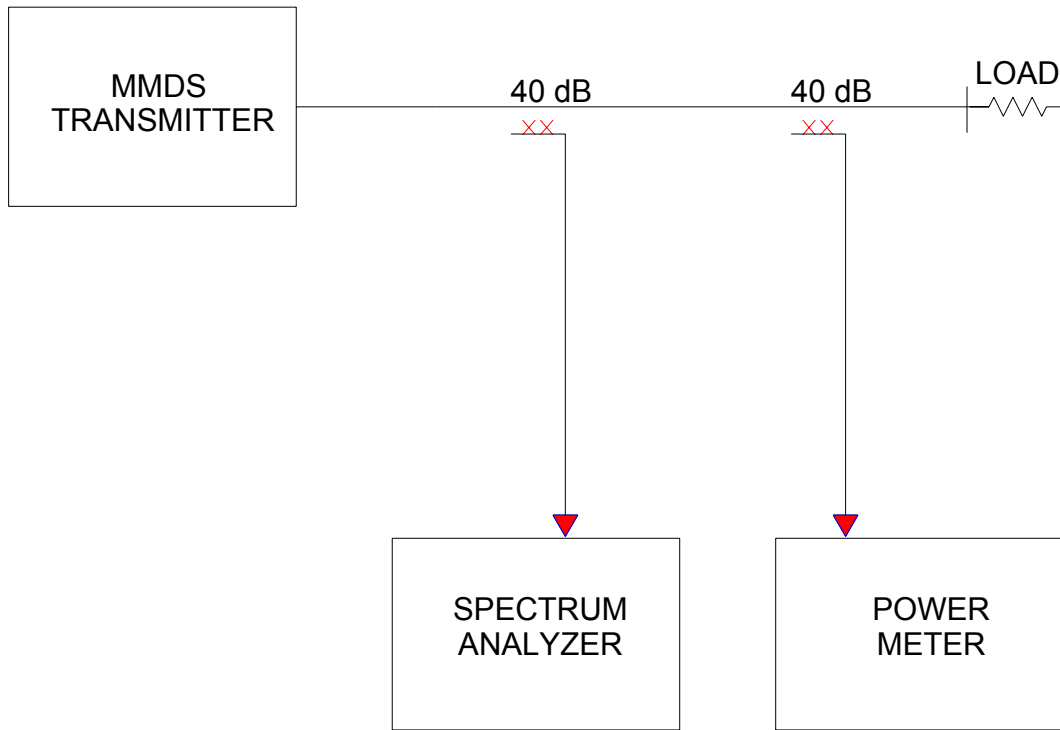
Figure 18. RF Power Measurement Set-up.
