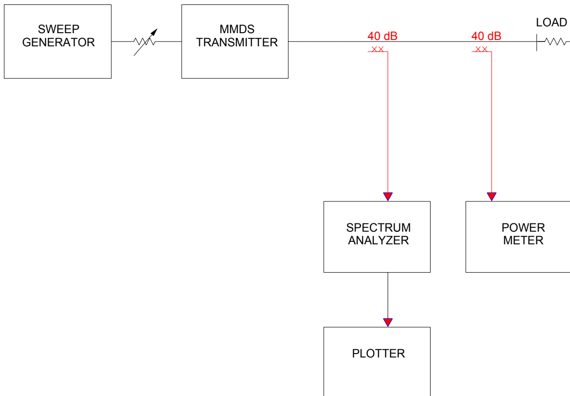
Figure 18. RF Power Measurement Set-up.
