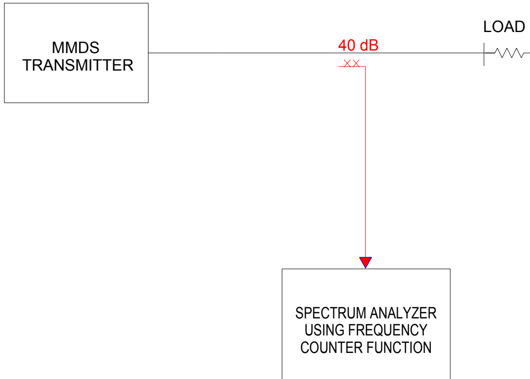
Figure 20. Frequency Stability Measurement Set-up.
