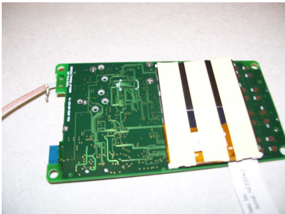
Figure 3 - Internal Photo, Underneath LCD
