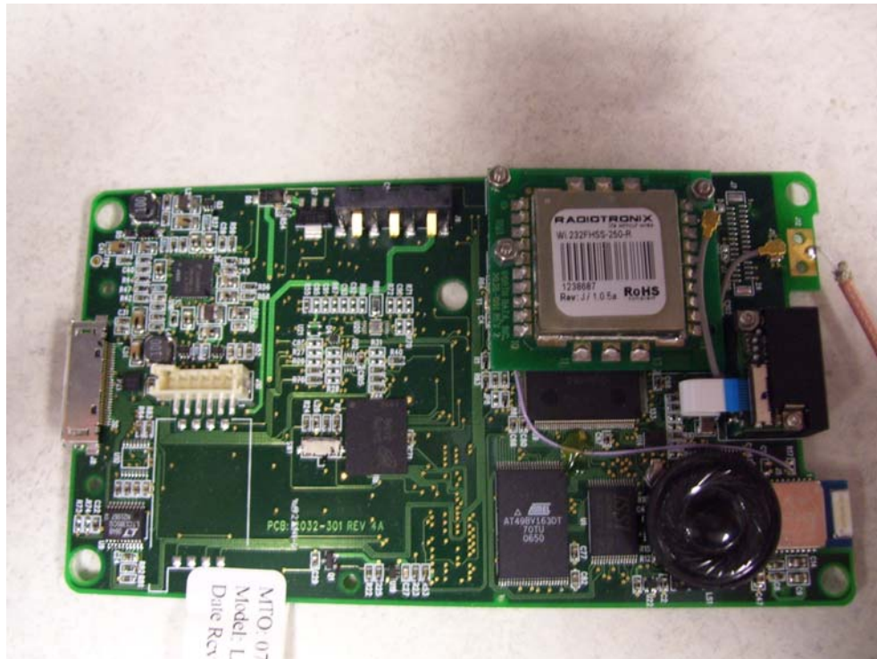
Figure 1 - LT7001H, Bottom Internal
