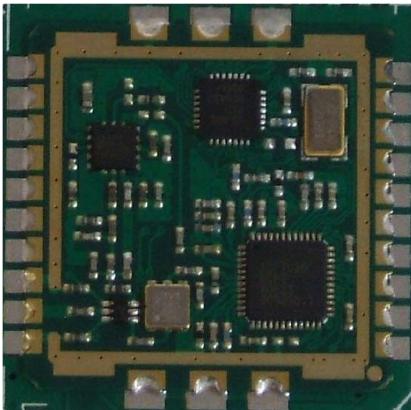
Figure 6 - Inside of Transmitter Module
