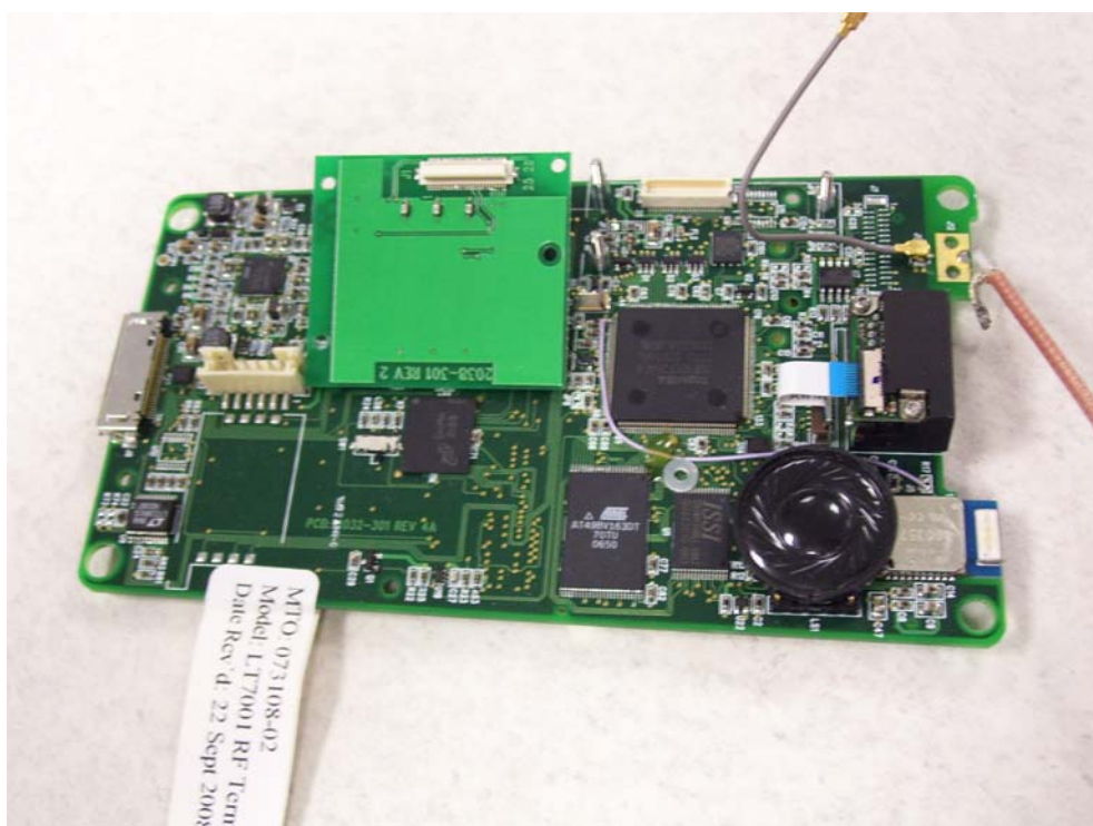
Figure 4 - Internal Photos, Underneath Transmitter Module
