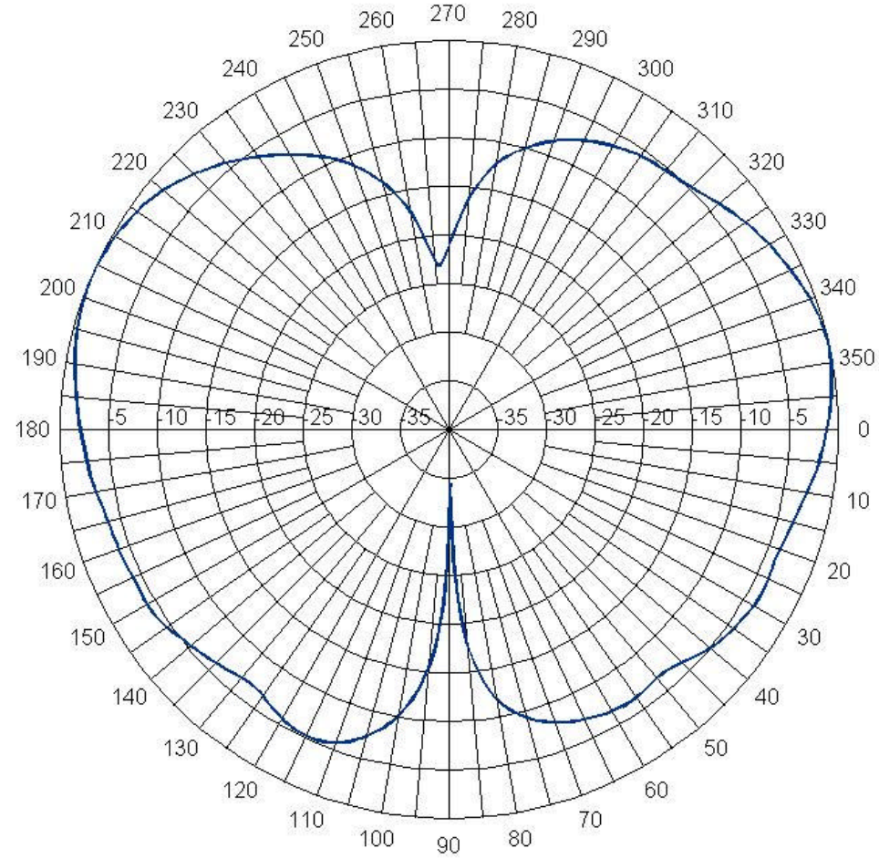
MAXRAD MEXE902 - Elevation Plane Radiation Pattern
