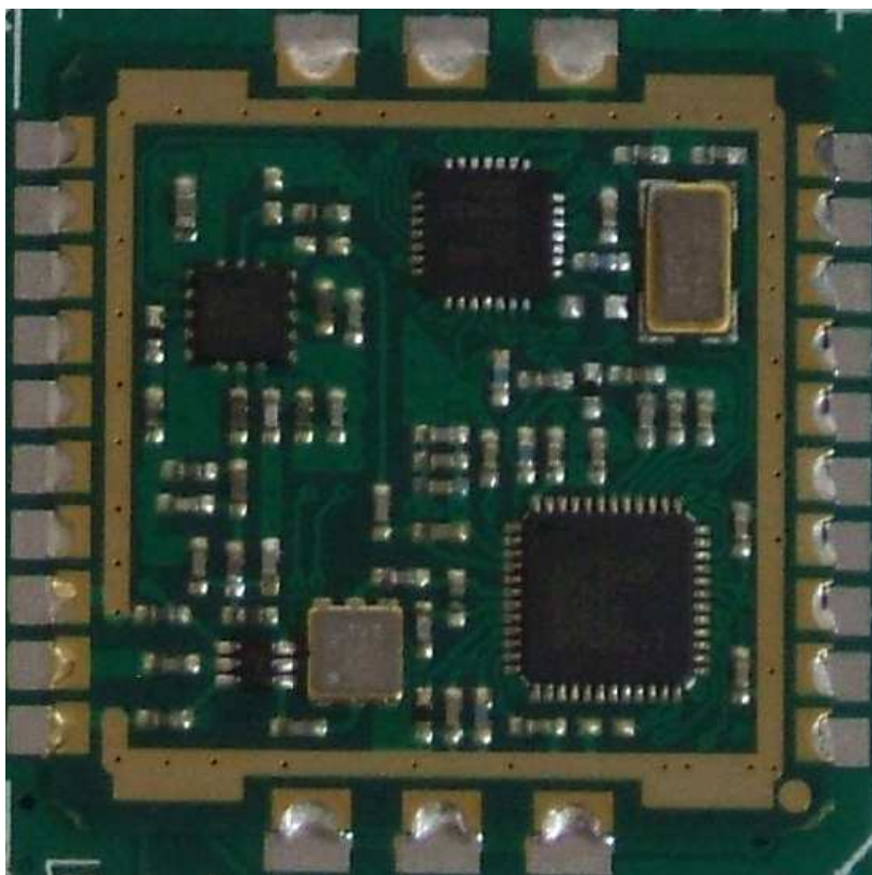
Figure 3 - Transmitter module with shield removed
