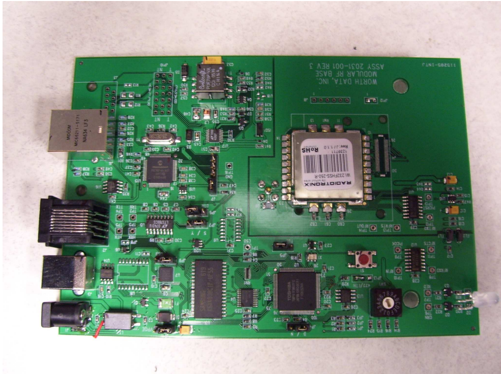
Figure 1 - B5002, Top Internal
