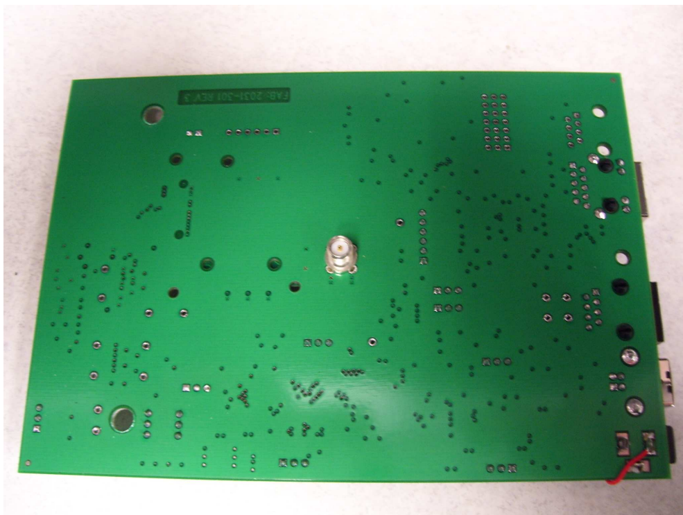
Figure 2 - B5002, Bottom Internal
