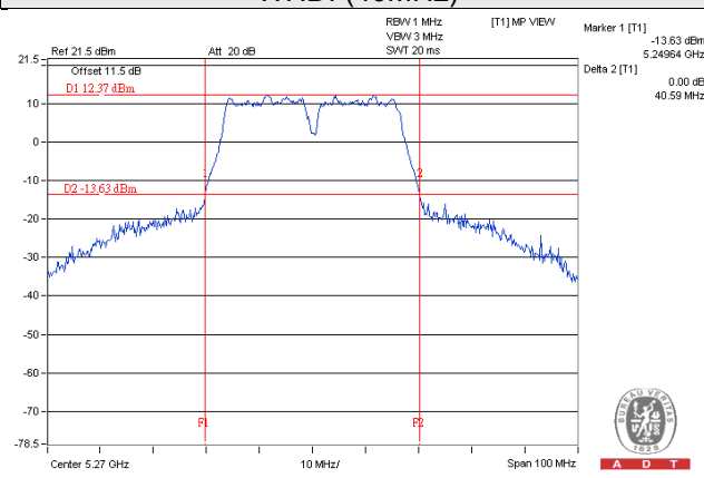
WHDI (40MHz)
