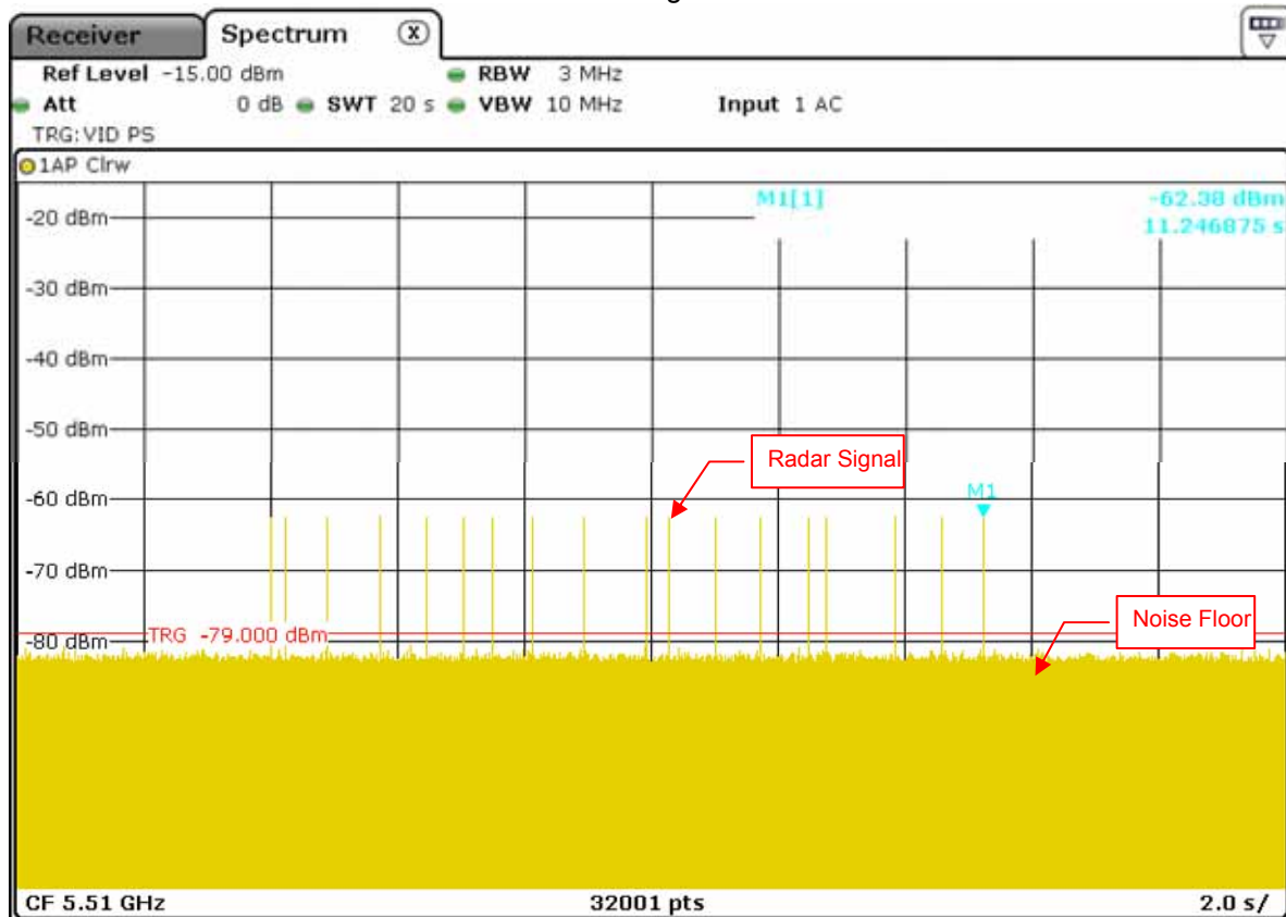
Radar Signal 5
