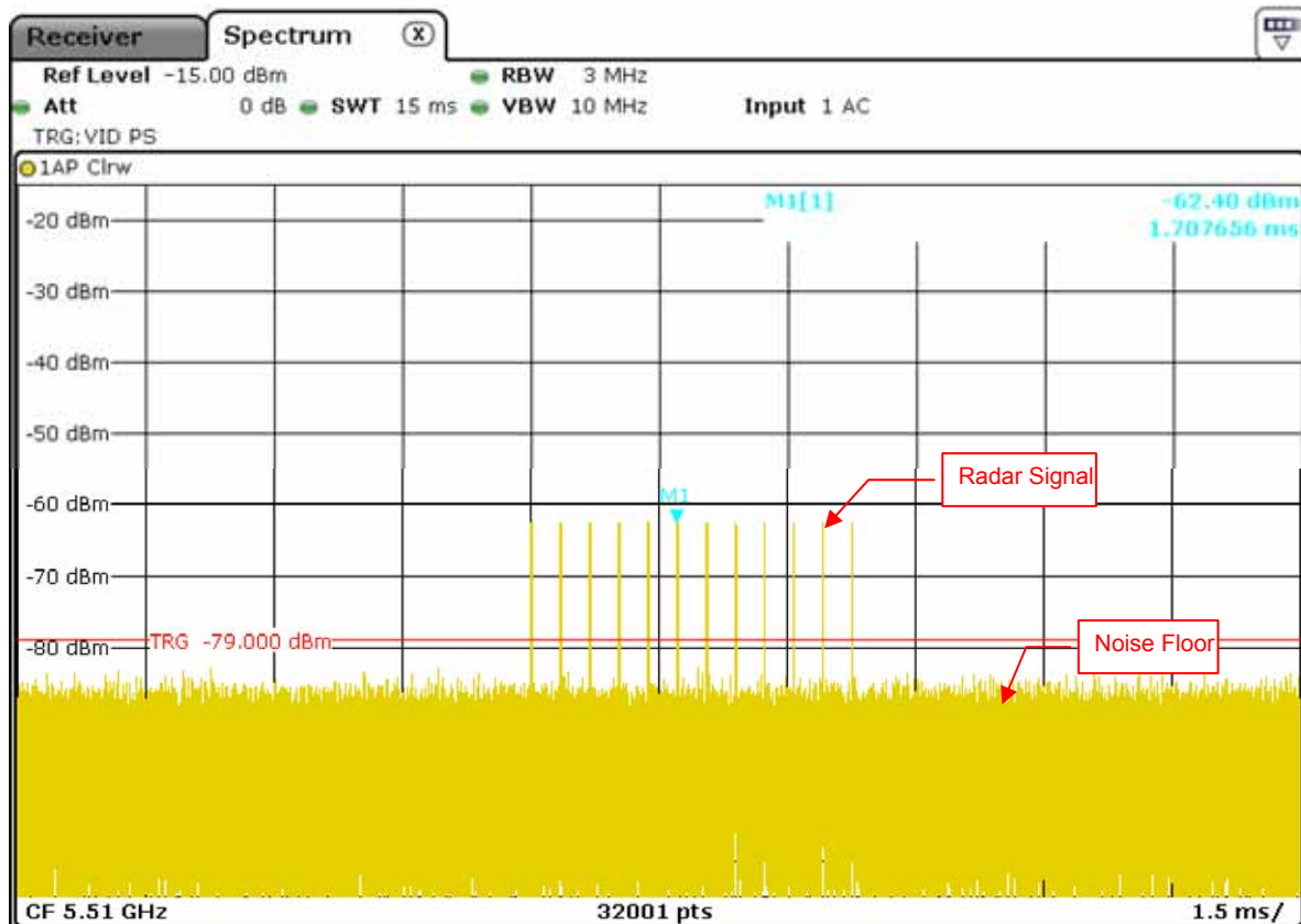
Radar Signal 4
