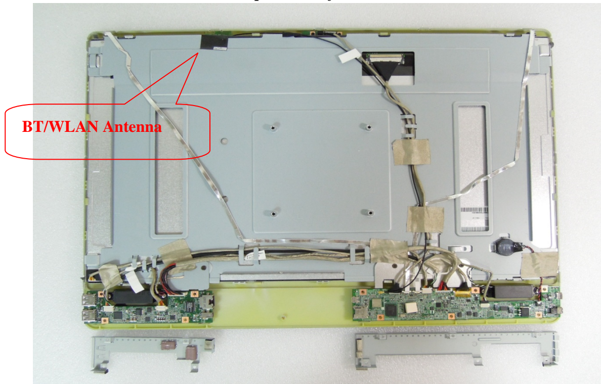
Open View of EUT –4
