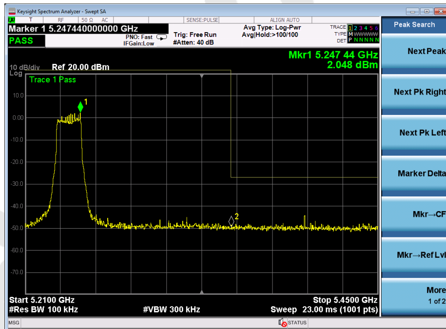
802.11n(20): Band Edge, Right Side
