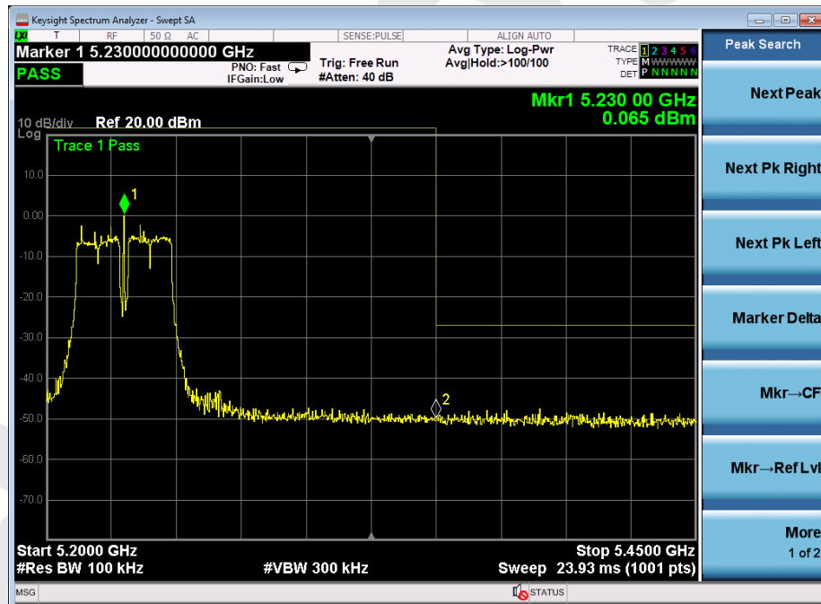
802.11ac(20): Band Edge, Right Side
