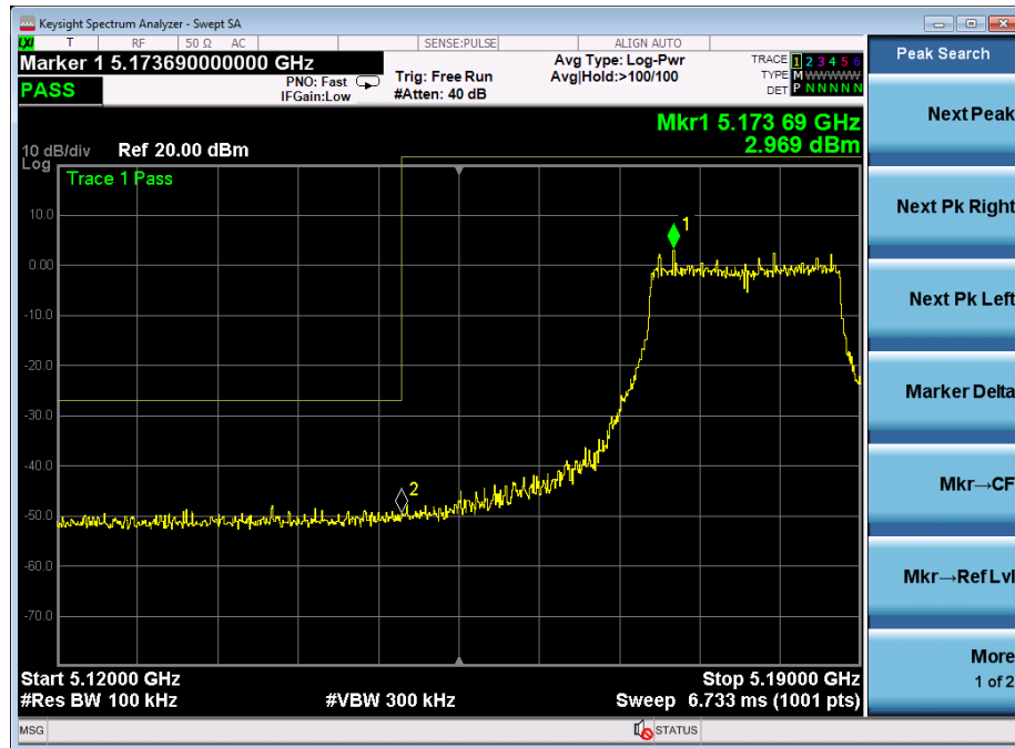
802.11n(20): Band Edge, Left Side
