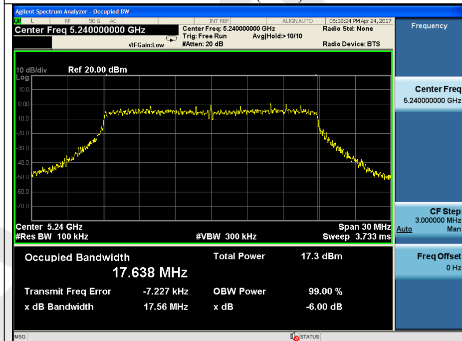
6dB Bandwidth Test Mode: 802.11n(HT20)--5240
