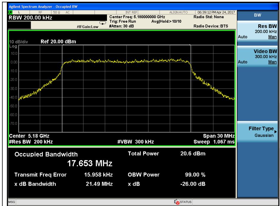
26dB & 99% Bandwidth Test Mode: 802.11a--5180
