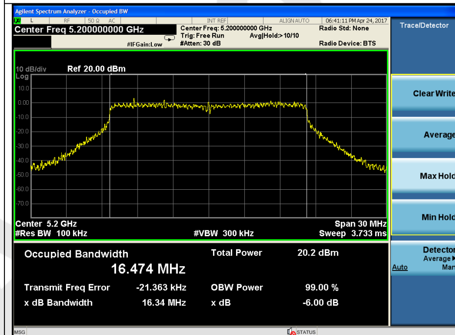
6dB Bandwidth Test Mode: 802.11a---5200
