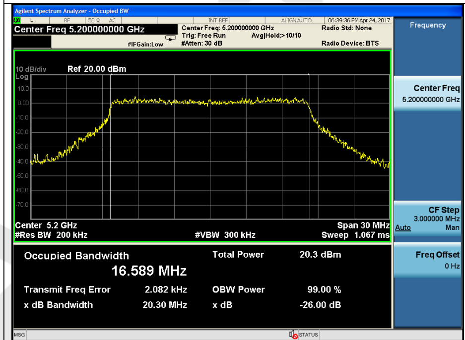
26dB & 99% Bandwidth Test Mode: 802.11a---5200
