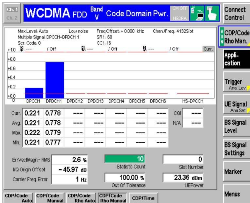
Single DPCCCH with only one DPDCH at RMC 12.2Kbps (Symbol Rate 60 Kbps)
