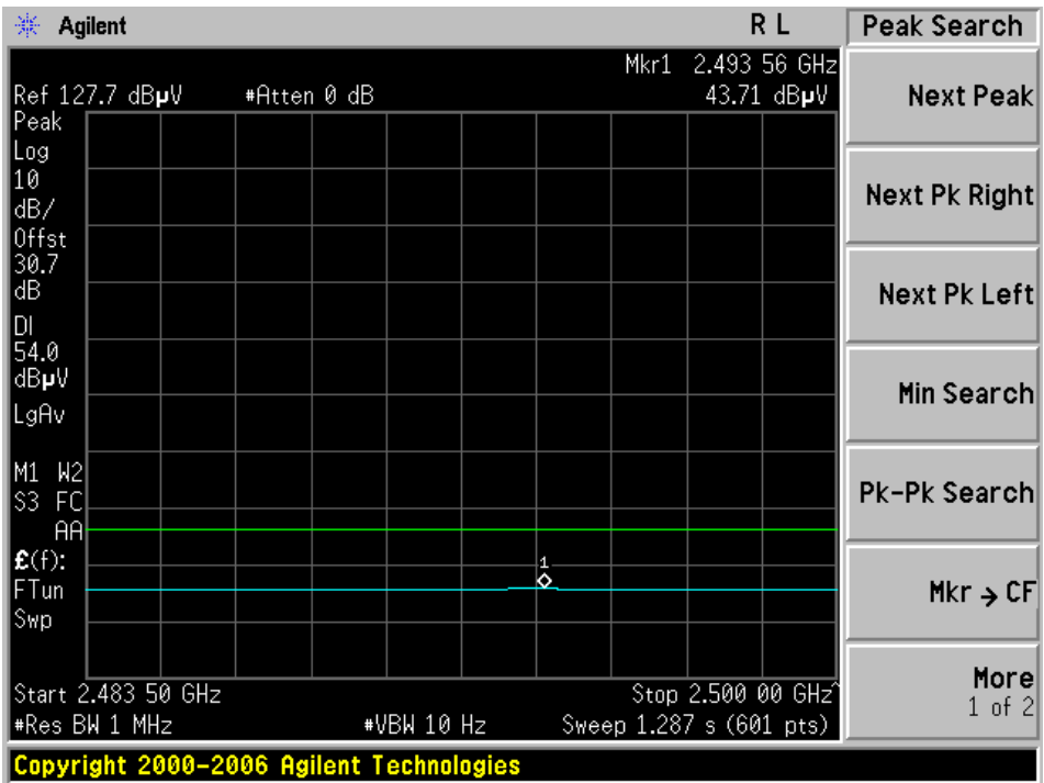
High Channel (2480 MHz), Vertical, Average
