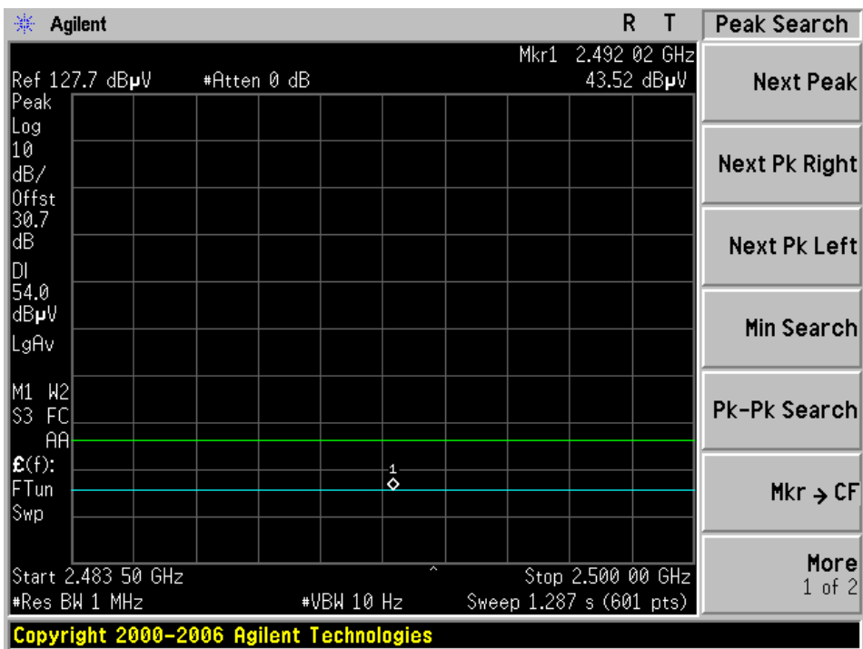
High Channel (2480 MHz), Horizontal, Average
