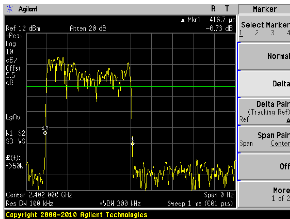
8PSK Mode, DH1, Low Channel
