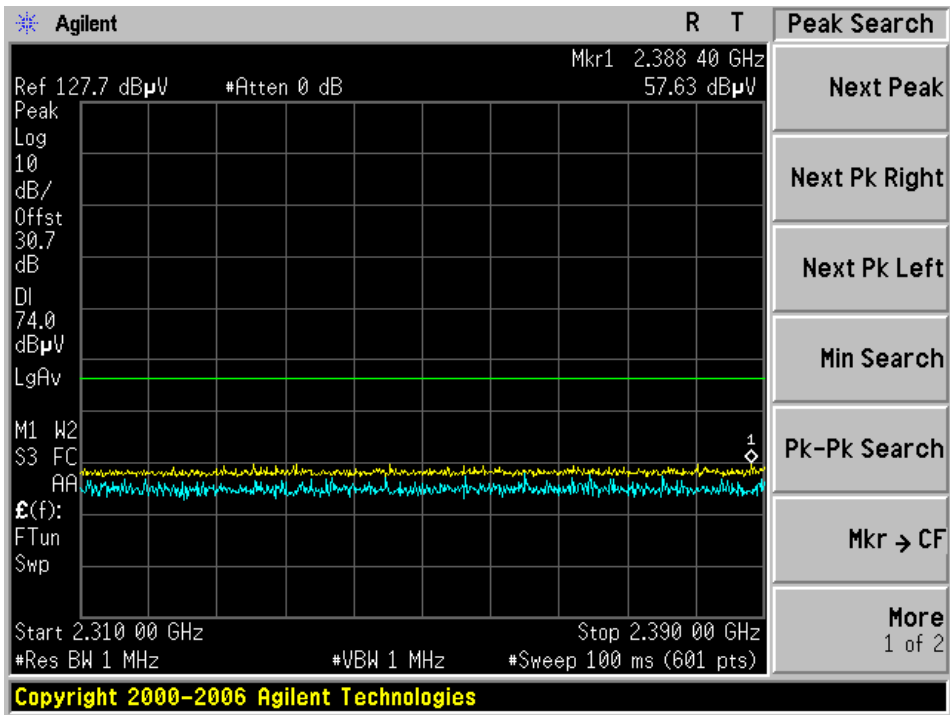
Low Channel (2402 MHz), Vertical, Average
