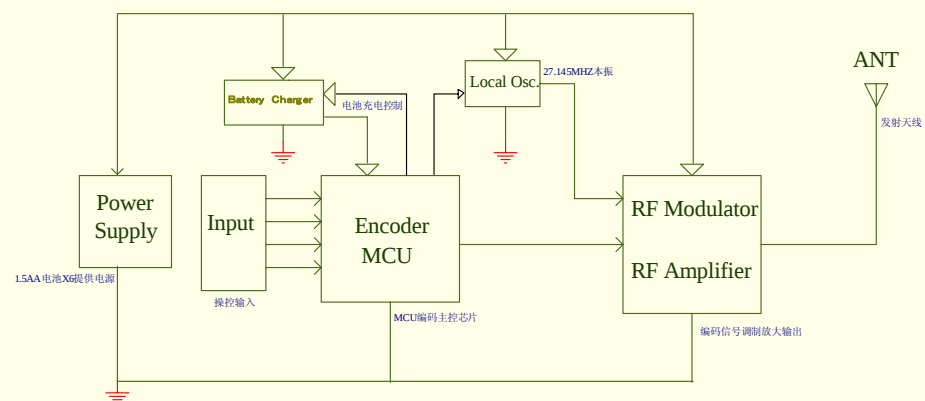
AM 27.145MHZ 22323 TX Block Diagram
