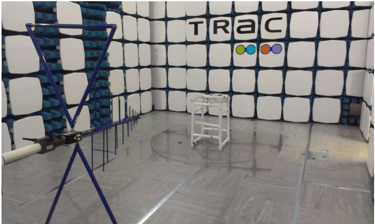
TRA-013040-02 Test set-up photos
