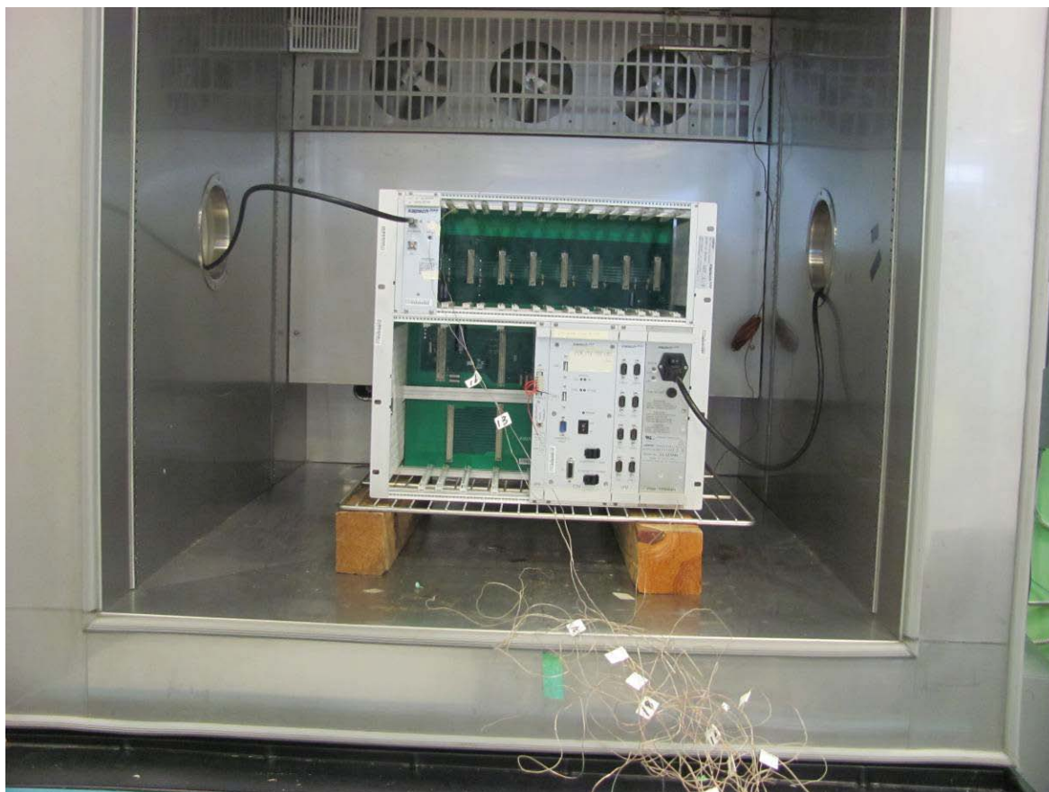
Illustration 6: Temperature stability setup - photo
