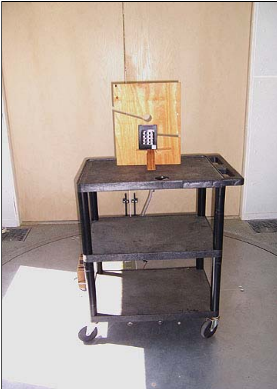
Radiated Emissions - Front View
