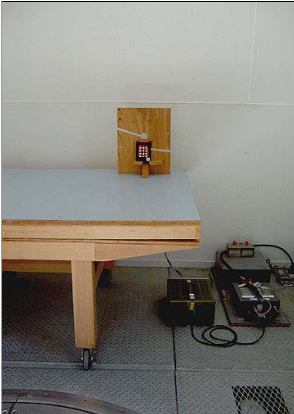
Mains Conducted Emissions - Front View
