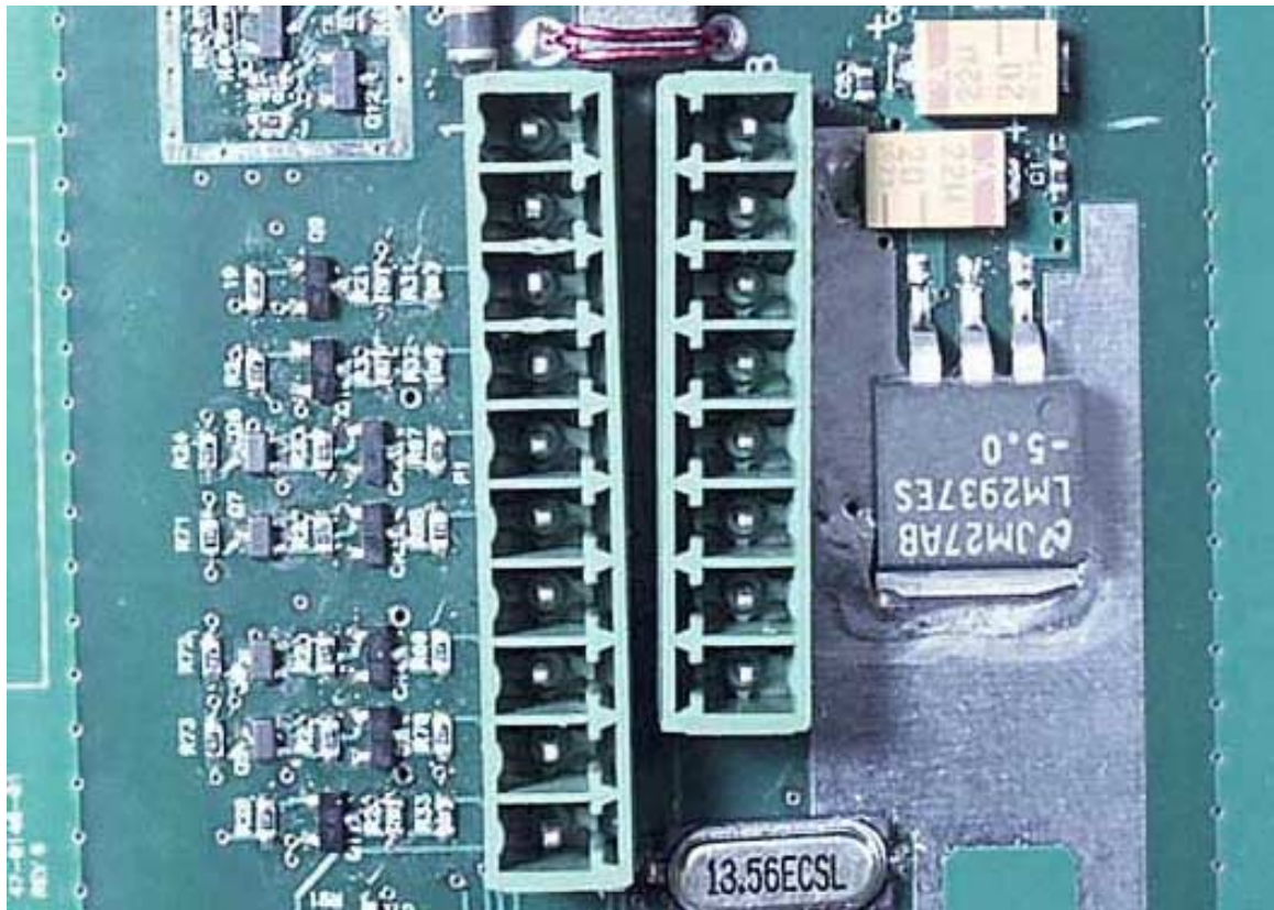
PCB Front Closeup 2
