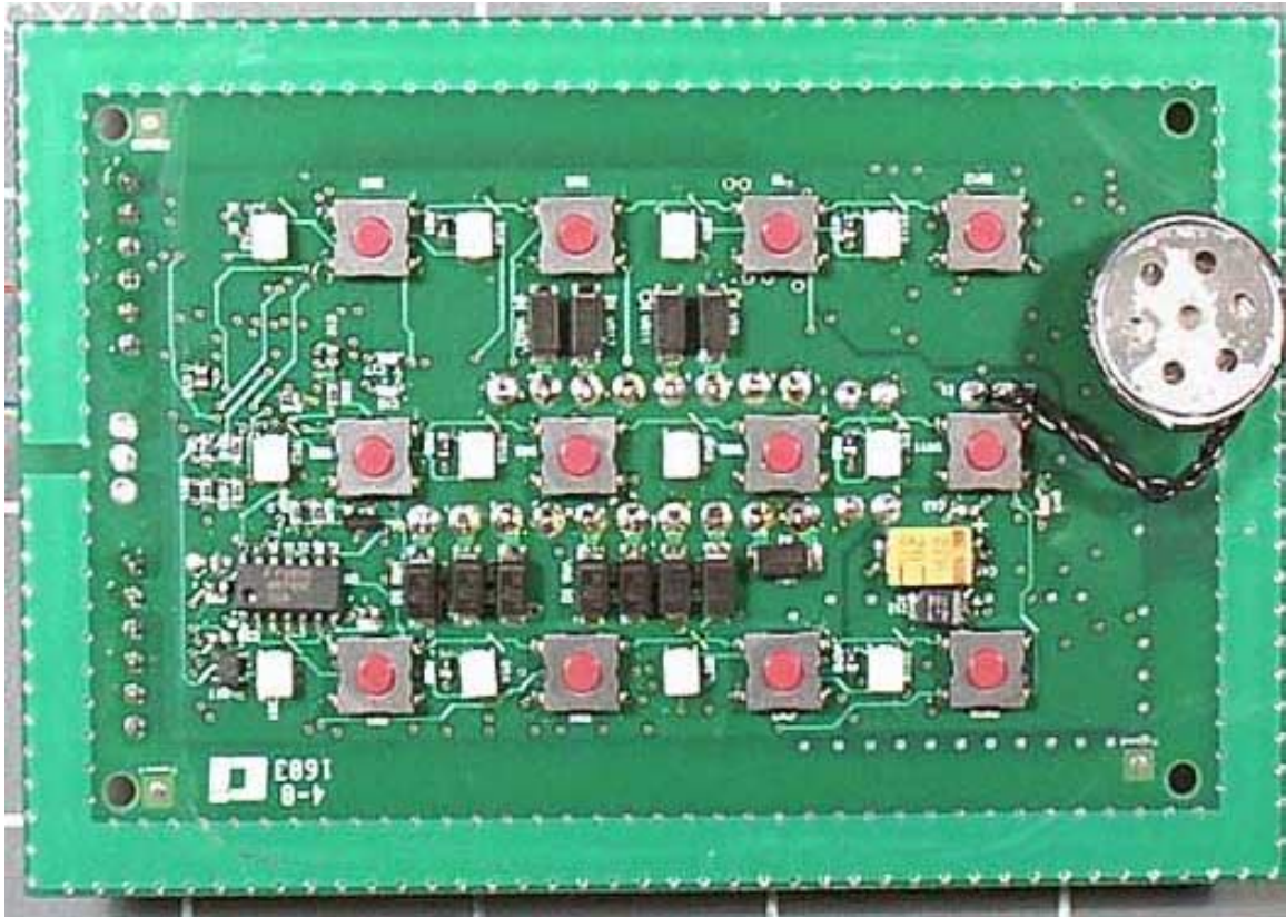
PCB Back Closeup
