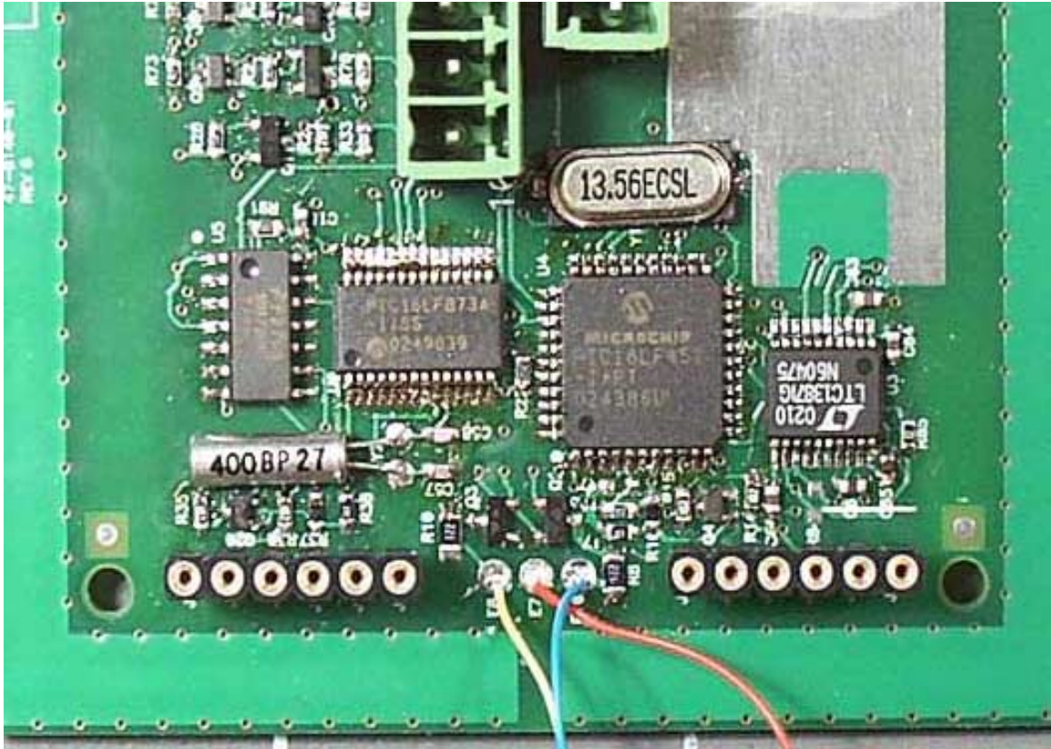
PCB Front Closeup 1
