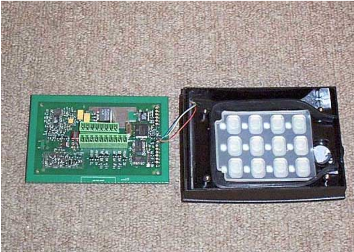
PCB Removed Front
