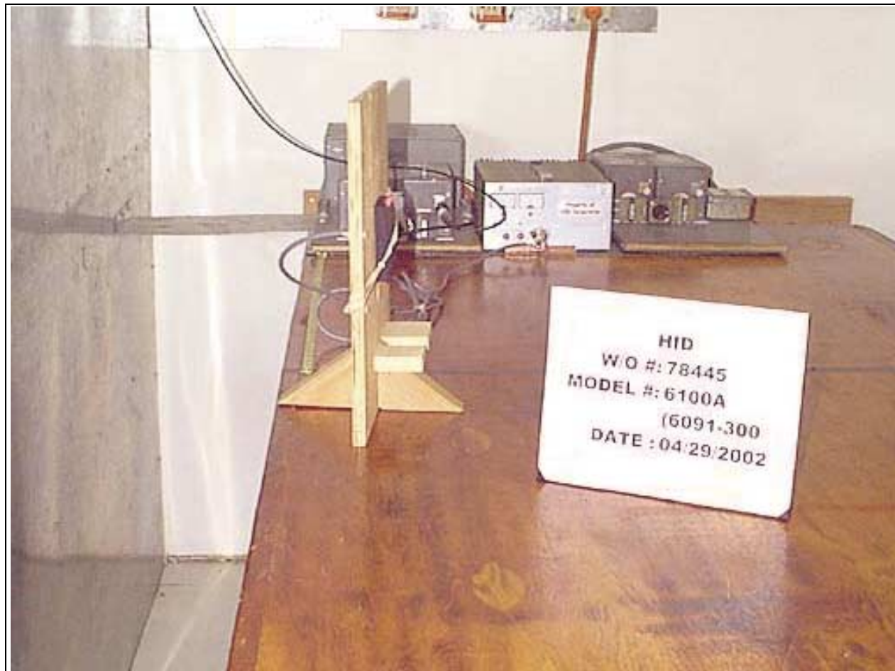
Mains Conducted Emissions - Side View - 6100A
