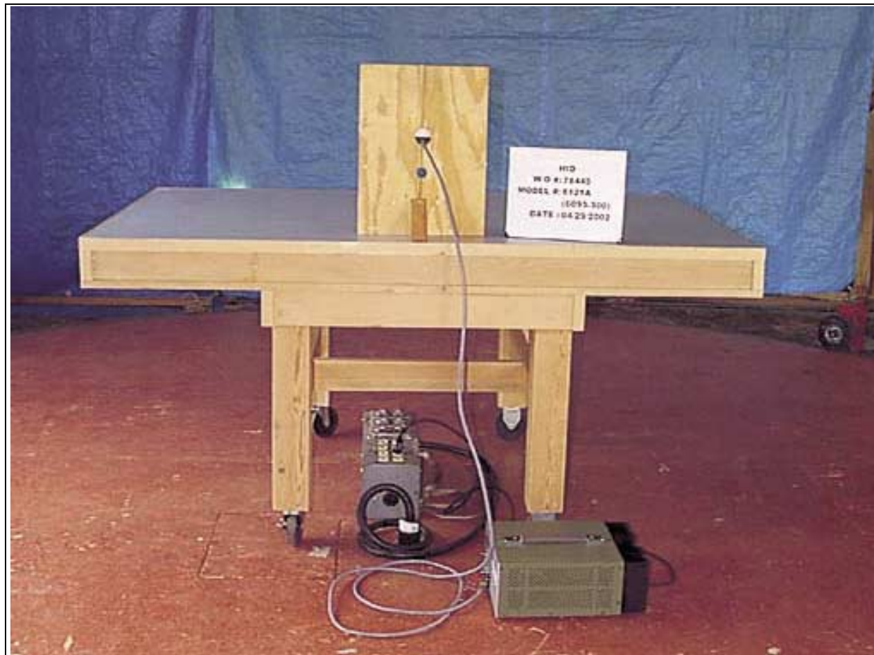
Radiated Emissions - Back View - 6121A
